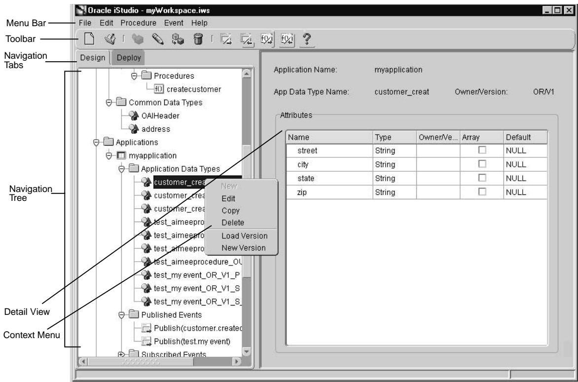
Figure 2–1 Oracle9iAS InterConnect iStudio
