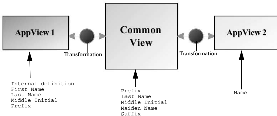
Figure 1-2 Oracle9iAS InterConnect Hub-and-Spoke Model
