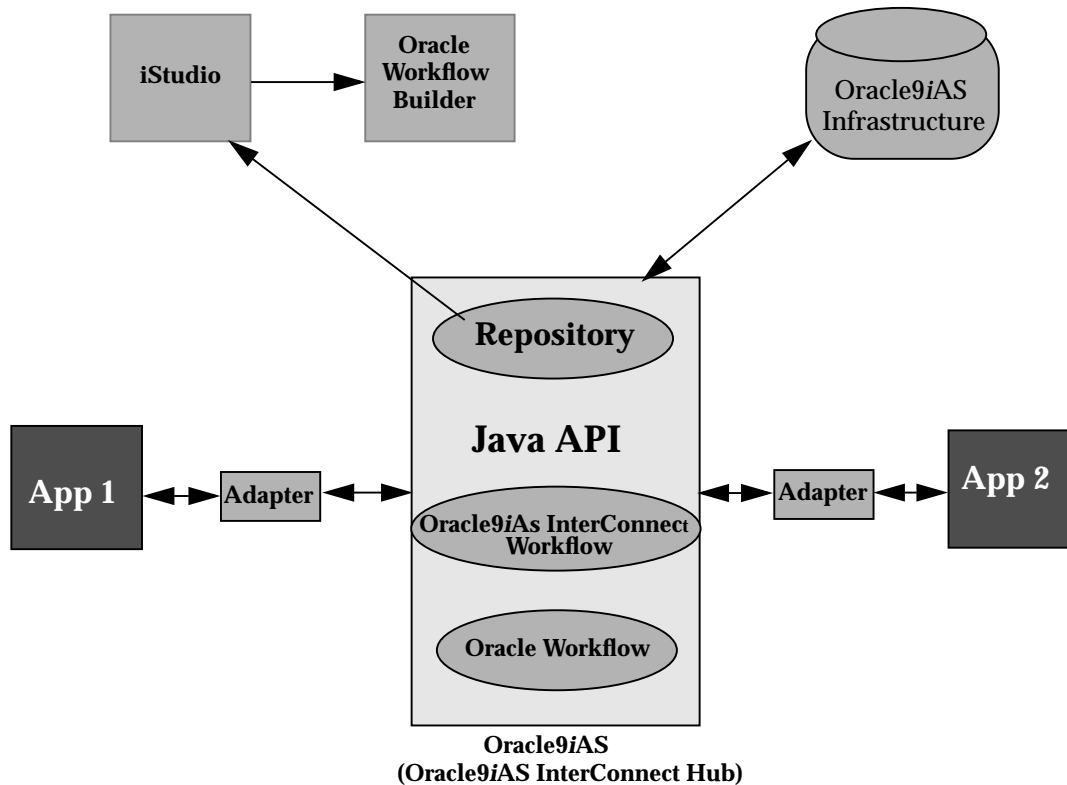
Figure 1–1 A graphical overview of design time and runtime phases in integration
