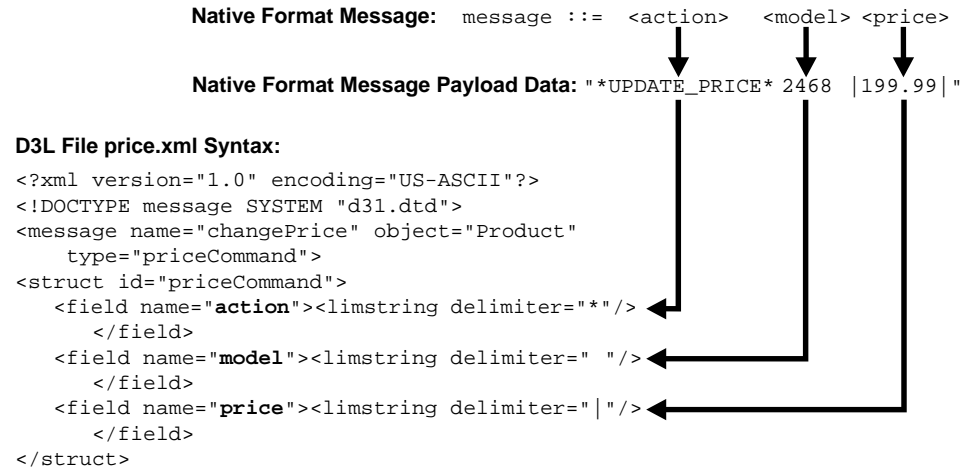
Figure B-1 Native Format Message Payload Data and D3L File Syntax
