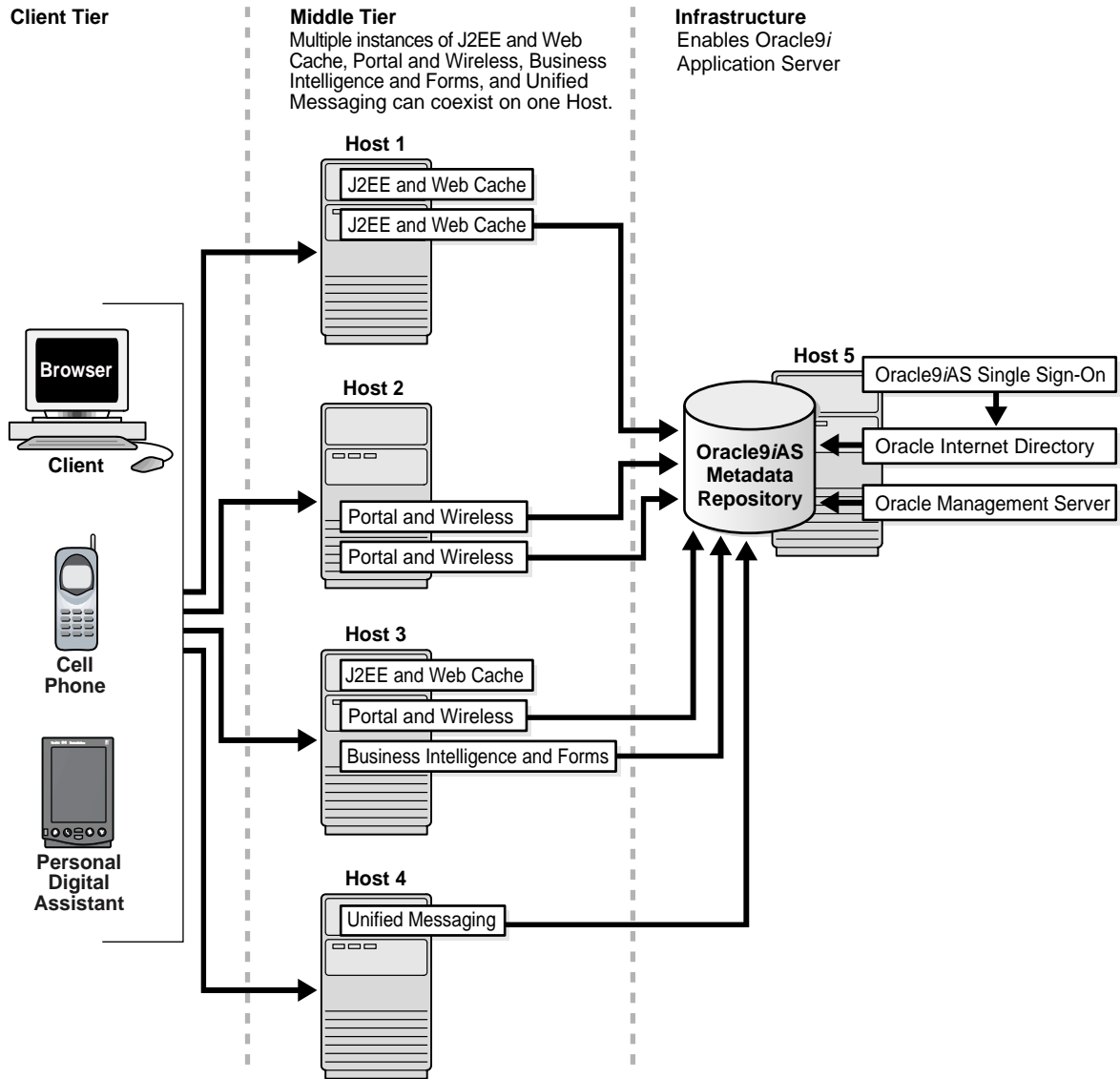
Figure 1-1 Oracle9iAS Architecture
