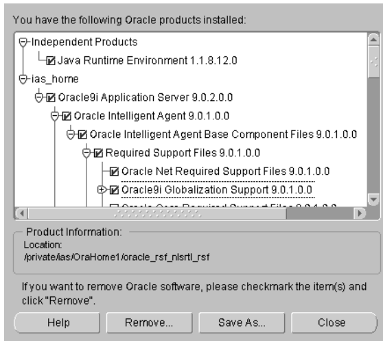
Figure 8–1 Inventory Screen
