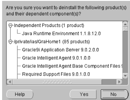
Figure 8–2 Confirmation Screen
