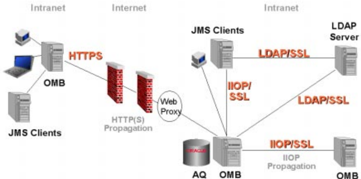
Figure 12-1 Sample Oracle Message Broker Deployment
