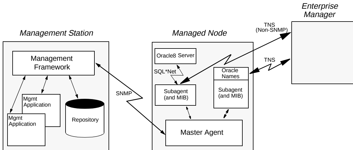
Figure 1–1 Basic Components of Oracle SNMP support.
