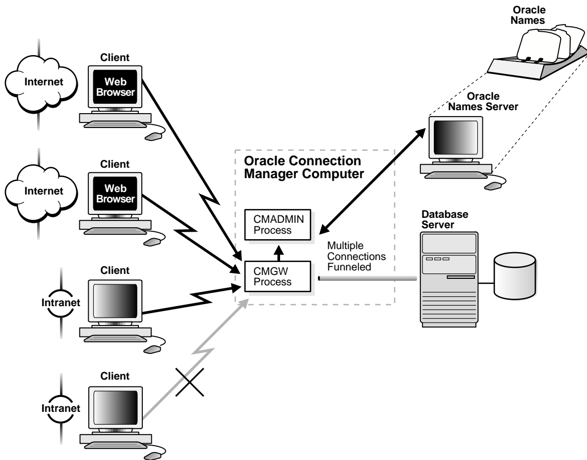
Figure 4-10 Oracle Connection Manager Architecture
