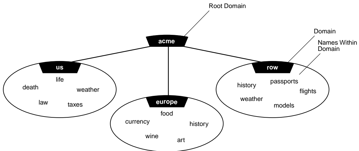
Figure 3–11 Hierarchical Naming Model
