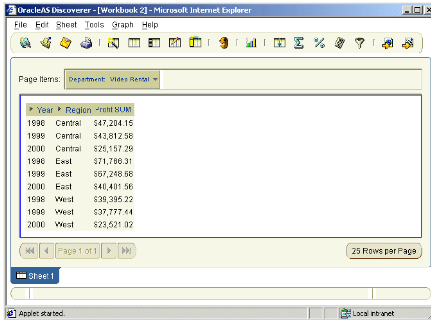
Figure 3–13 Sheet 1 worksheet
