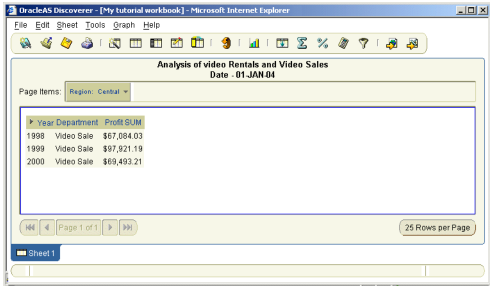
Figure 3–31 Worksheet with Profit SUM > 50000 condition applied
