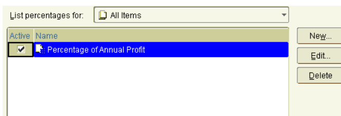
Figure 4–18 Percentages list
