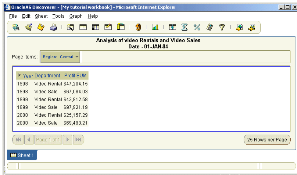
Figure 3–26 Sheet 1 worksheet
