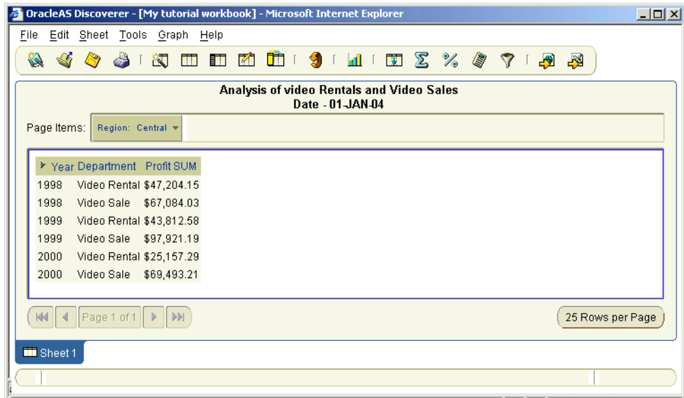
Figure 3–38 Sheet 1 worksheet
