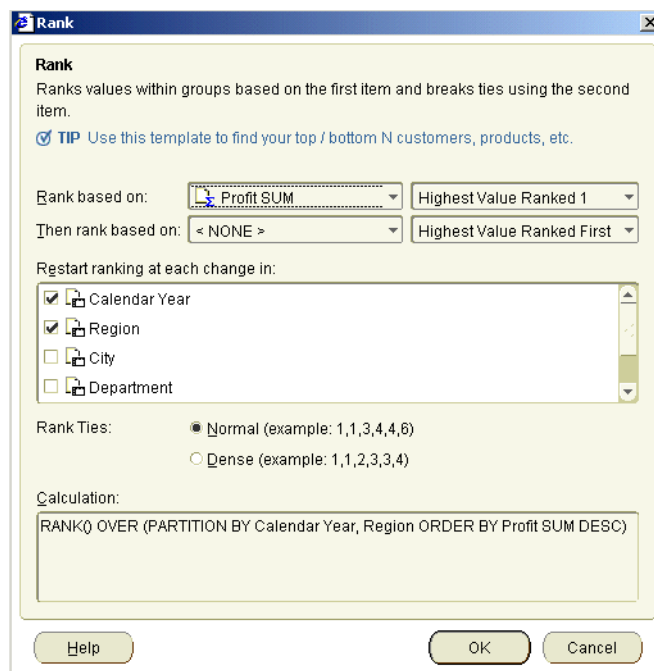
Figure 4–27 Rank dialog
