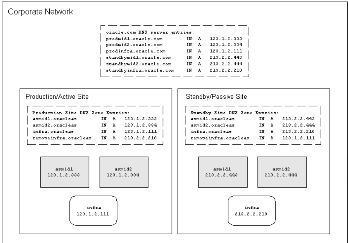
Figure 6–3 DNS resolution topology overview
