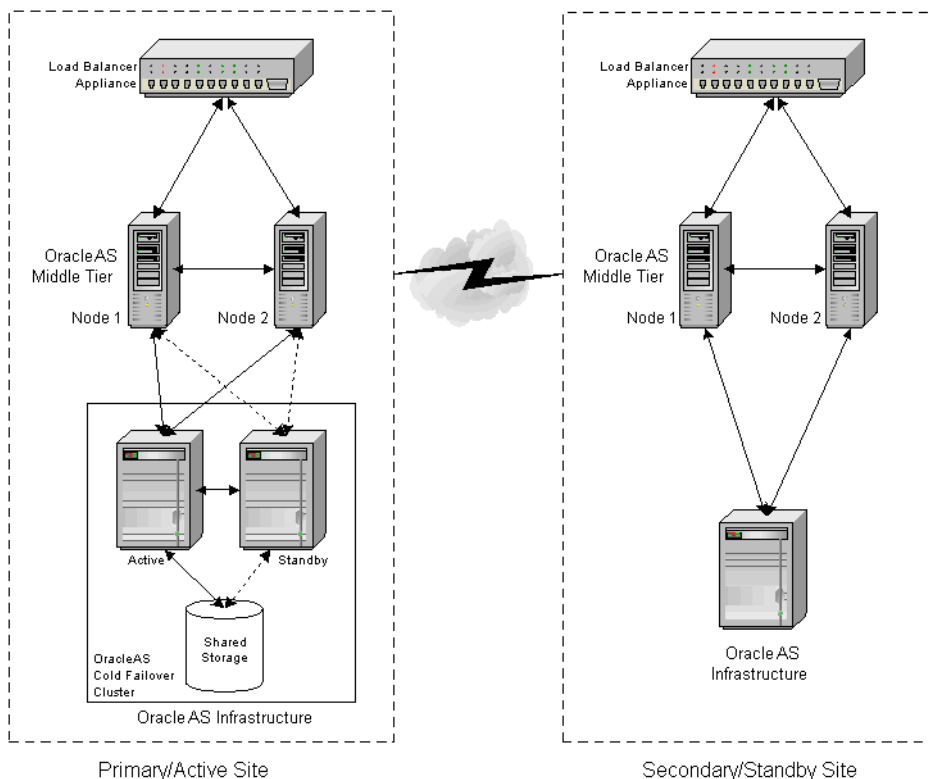
Figure 6–1 Oracle Application Server site-to-site disaster recovery solution (load balancer appliance is optional if only one middle tier node is present)
