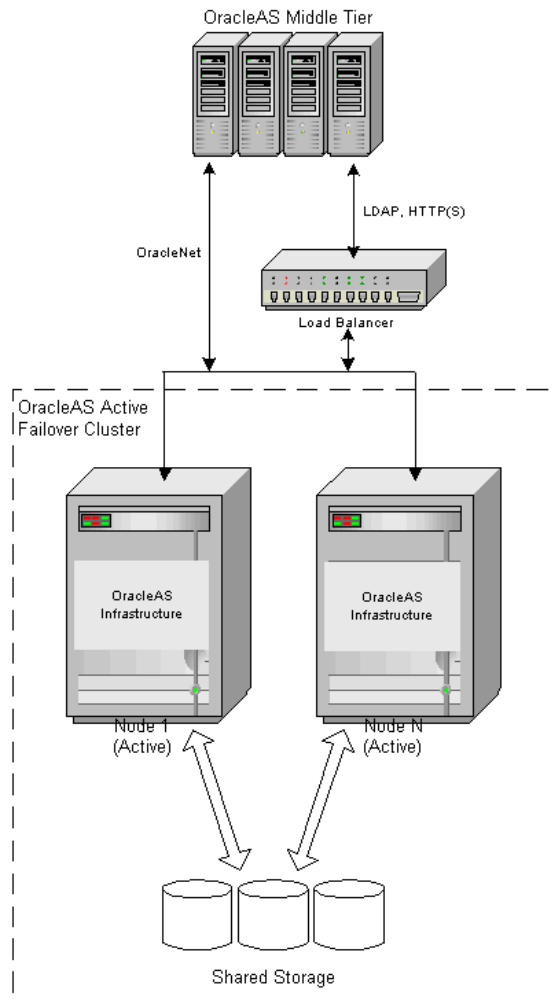
Figure 3–4 OracleAS Active Failover Cluster high availability solution
