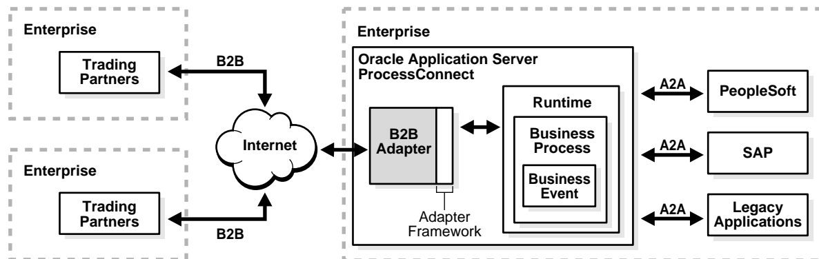
Figure 4–2 Oracle Application Server ProcessConnect Technology Adapter Overview
