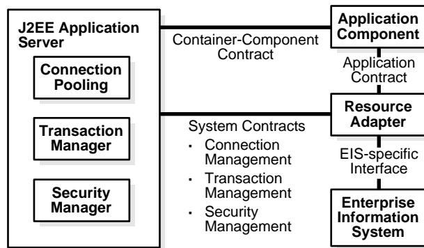
Figure D-1 J2EE Connector Architecture
