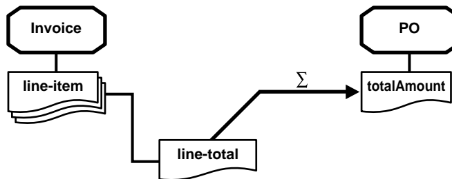
Figure 14–11 Cumulative Computation
