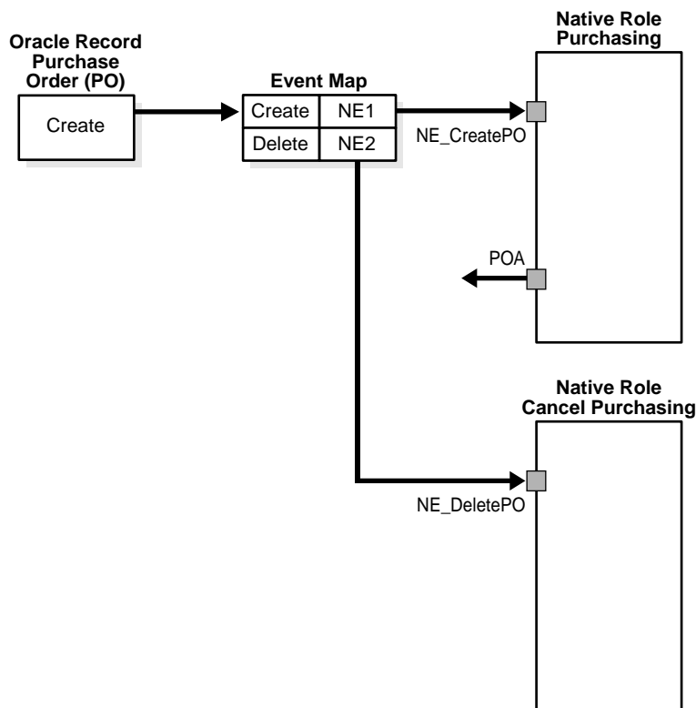
Figure 11–8 Event Mapping
