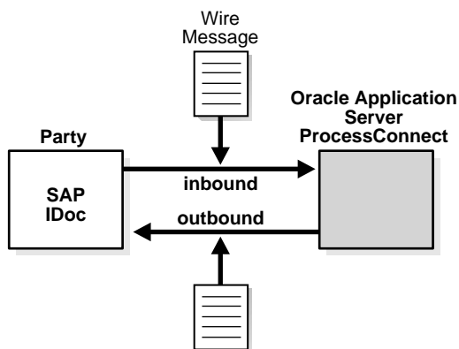
Figure 3–1 Wire Message
