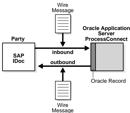
Figure 3–2 Oracle Record
