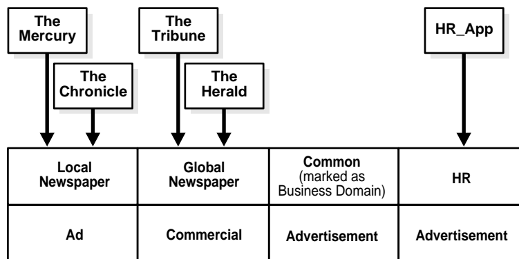
Figure 14-15 Domain-Party Relationship
