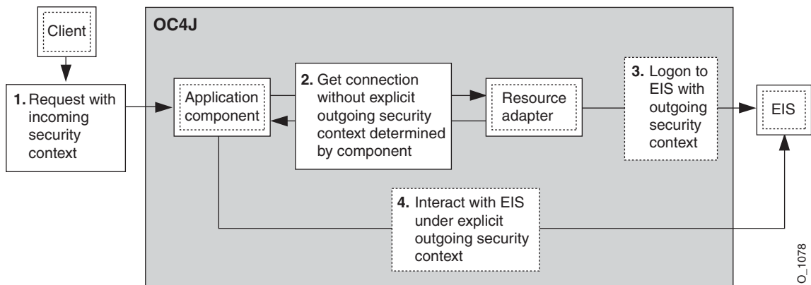
Figure 8–2 Component-Managed Sign-On
