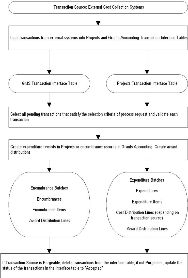
Figure B–1 Transaction Import Process Diagram
