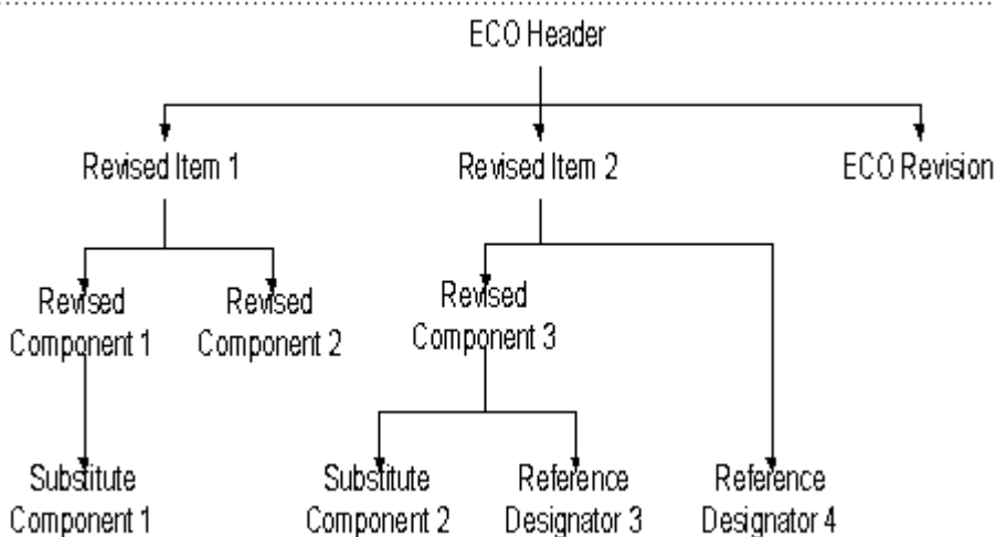
Figure 6–2 Business Object Interface Design
