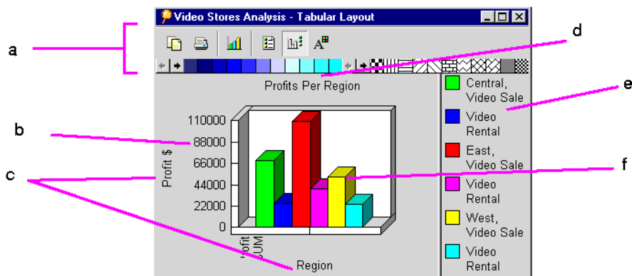
Figure 3–2 Graph Window
