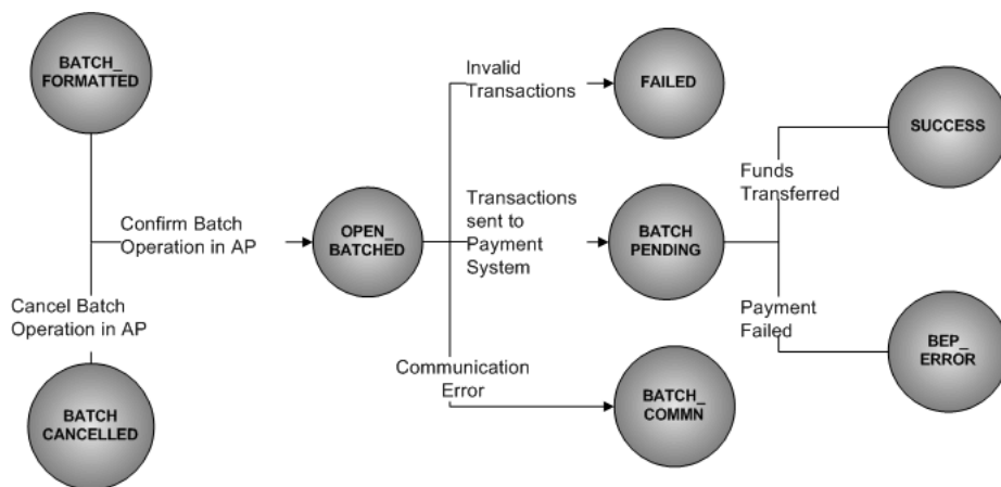
Figure 1–4 Outbound Payment Transaction Status
