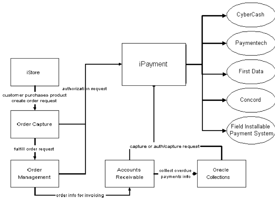
Figure 1-1 iPayment's Integration with Oracle Applications
