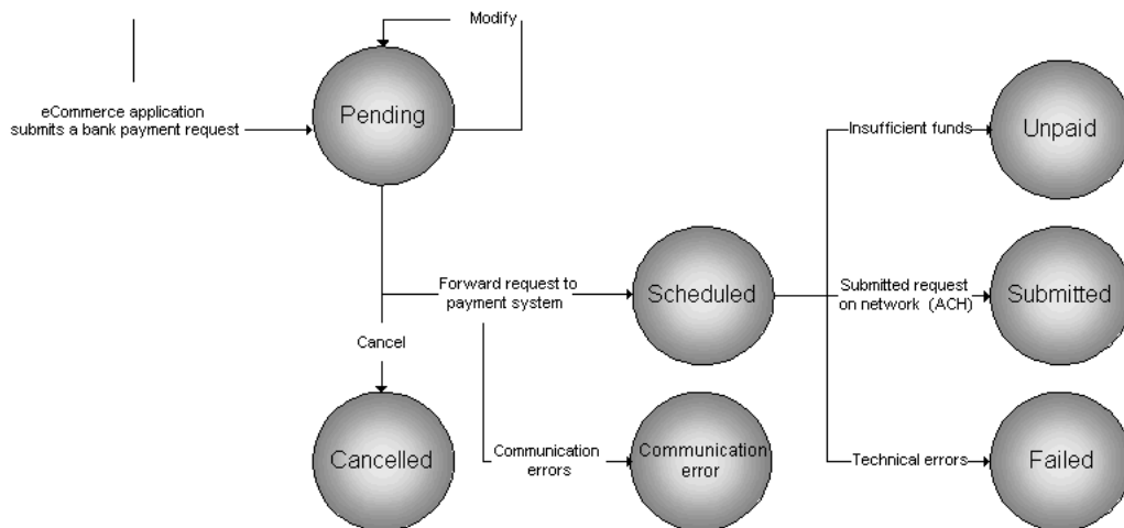
Figure 1-3 State Transition Diagram of an Inbound Bank Remittance
