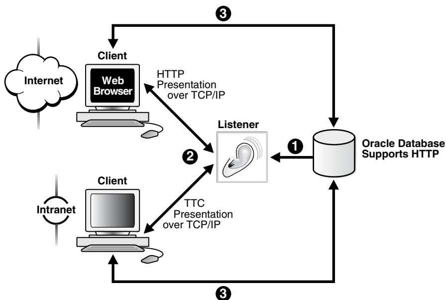
Figure 4-7 Listener Architecture
