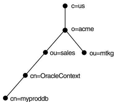
Figure 3–6 X.500 Style DIT
