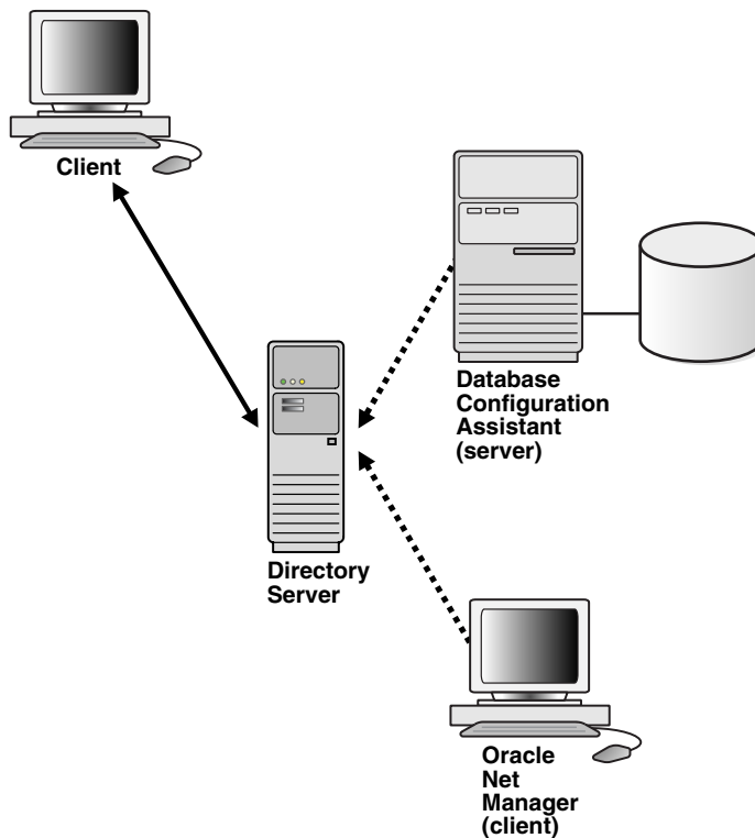
Figure 3–7 Creating Entries in the Directory Server with Applications
