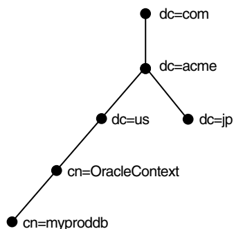
Figure 3–5 Domain Component DIT
