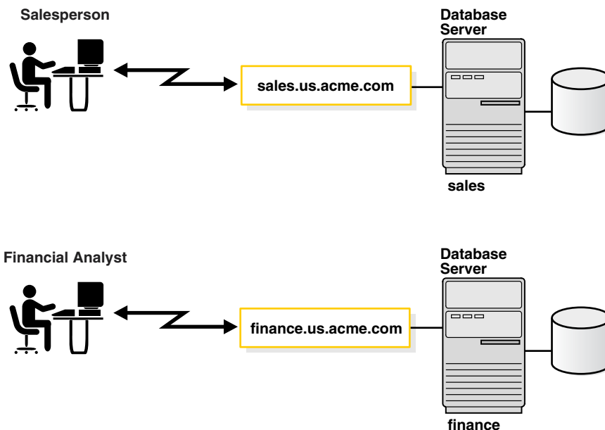
Figure 2–3 One Instance for each Database
