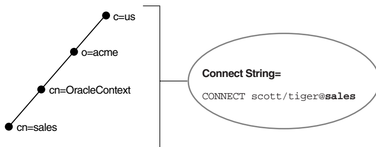
Figure 3–8 Relative Naming
