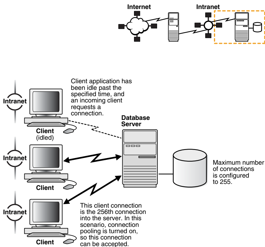
Figure 1-11 Connection Pooling
