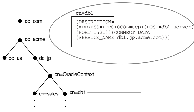
Figure 3–2 Database Service and Net Service Entries in a DIT
