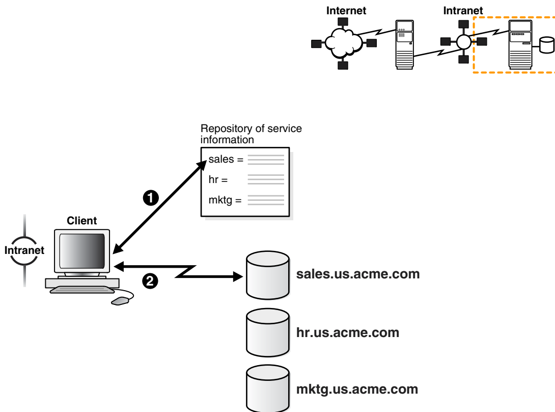
Figure 1-7 Service Information Repository
