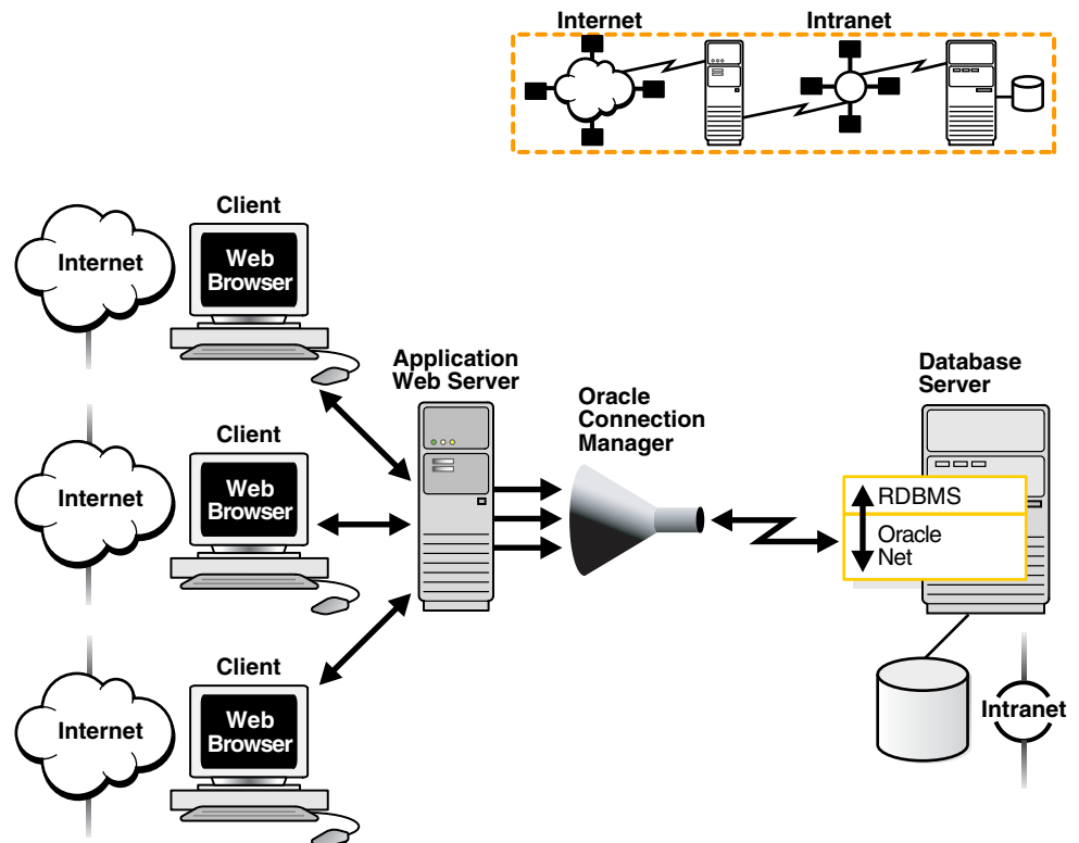
Figure 1–12 Session Multiplexing
