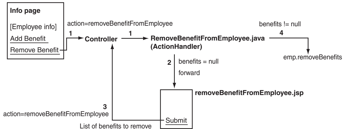
Figure 6–6 Remove Benefits Operation
