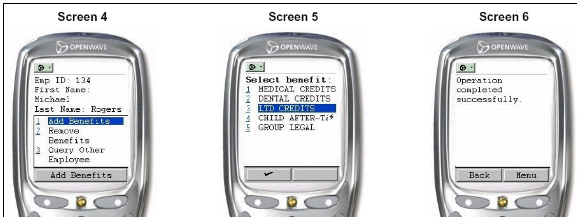
Figure 8-2 Screens for the Wireless Application (2 of 3)
