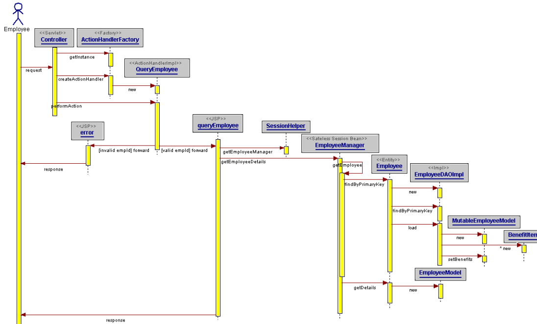
Figure 6–3 Sequence Diagram for Query Employee
