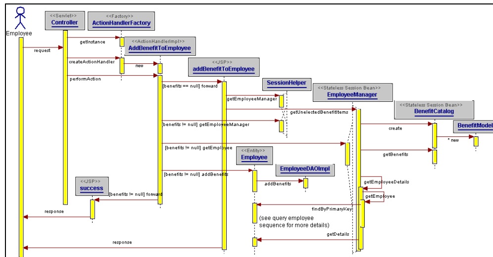
Figure 6–5 Sequence Diagram for Adding Benefits
