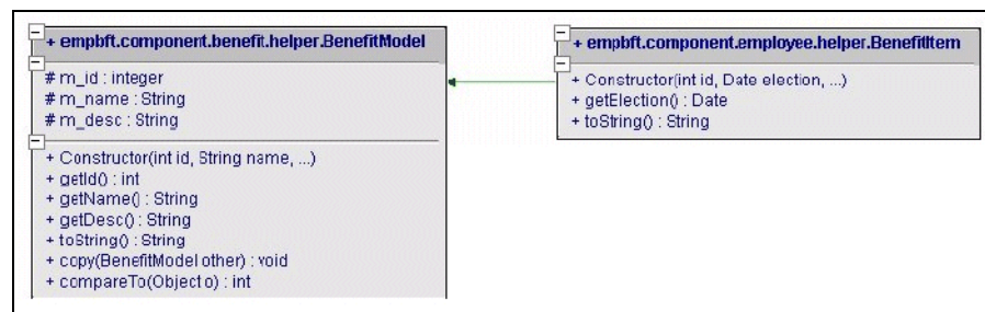
Figure 4–8 BenefitItem and BenefitModel Classes
