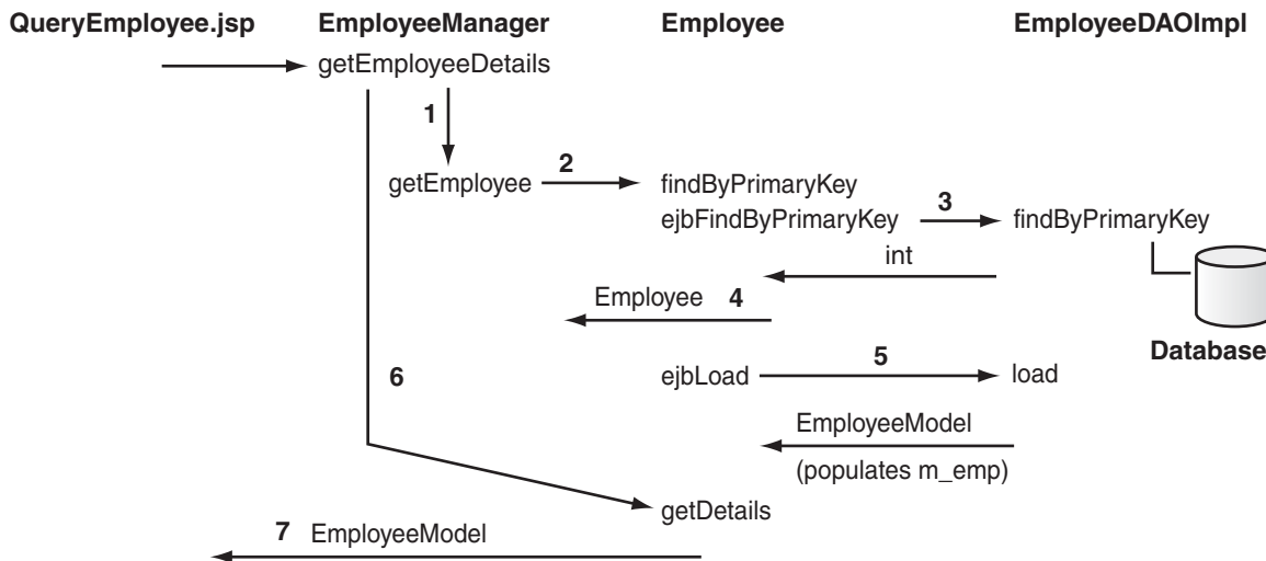
Figure 6–2 getEmployeeDetails
