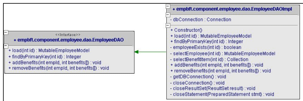
Figure 4-6 EmployeeDAO Classes
