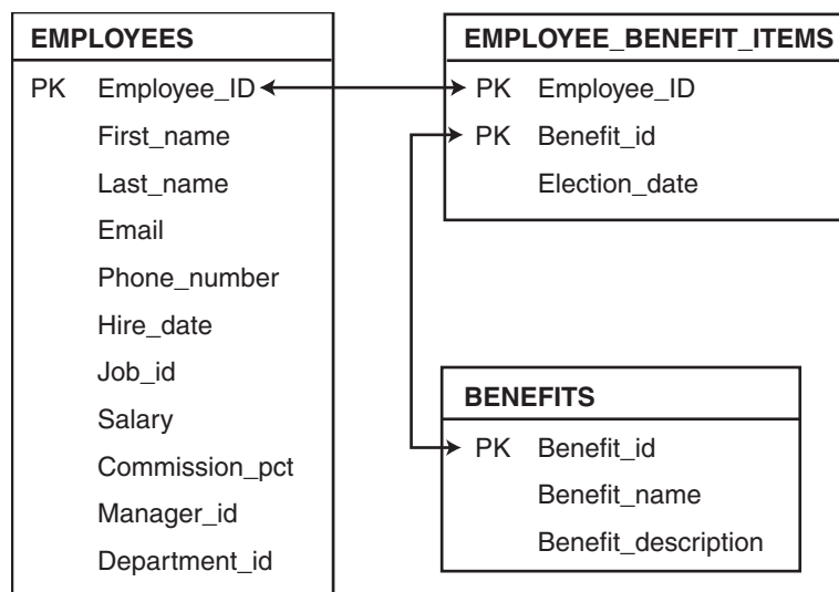
Figure 1-3 Database Schema
