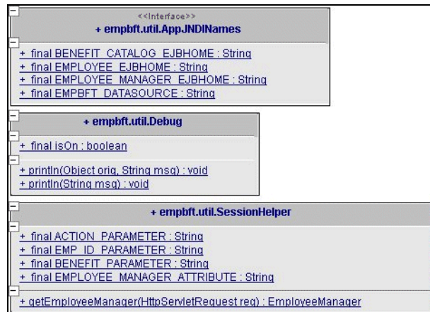
Figure 4–10 Utility Classes
