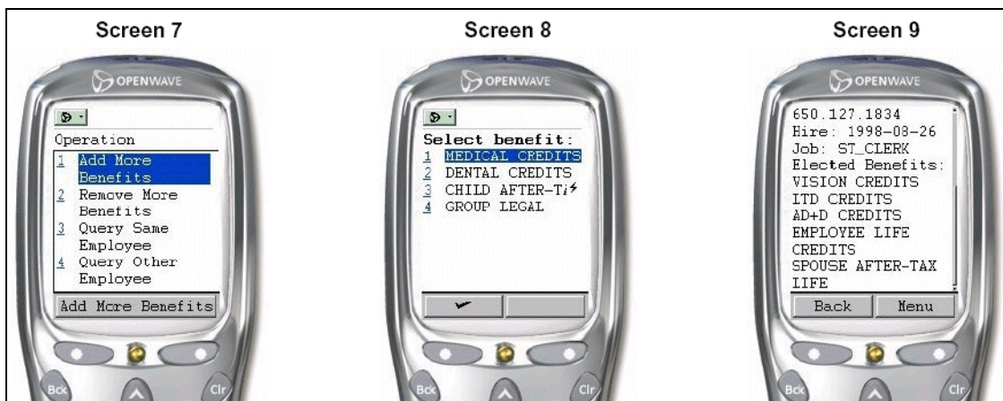
Figure 8-3 Screens for the Wireless Application (3 of 3)
