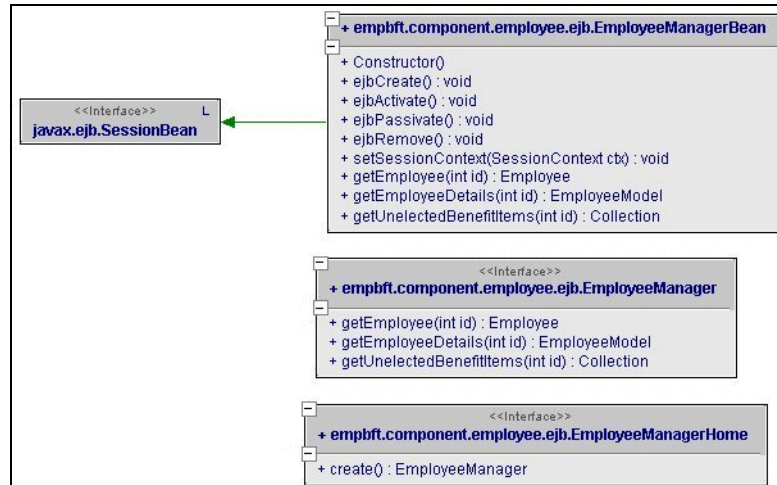
Figure 4–9 EmployeeManager Classes
