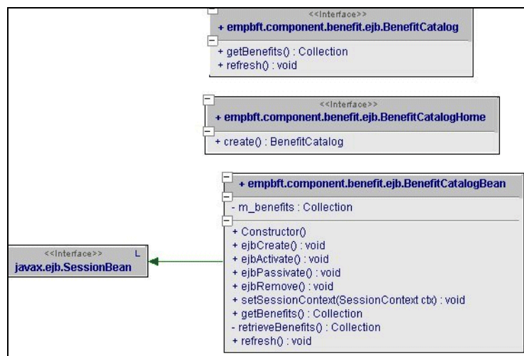
Figure 4–7 BenefitCatalog Classes
