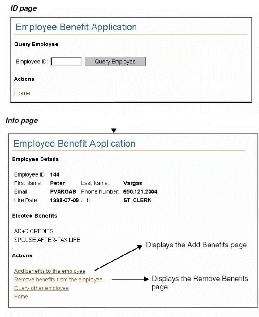
Figure 3–1 ID page and Info page
