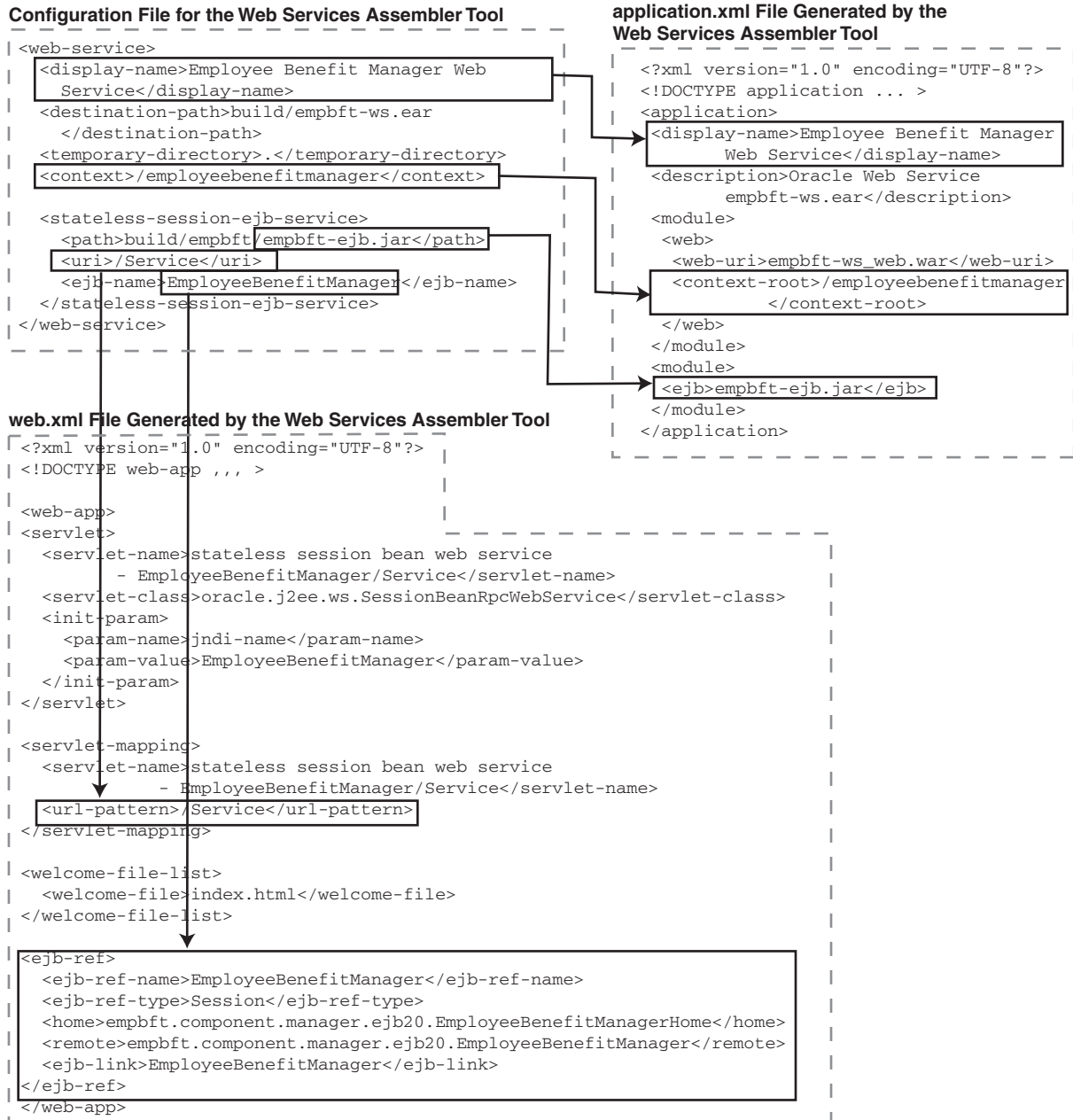
Figure 11–1 How the Web Services Assembler Tool Generates the application.xml File
