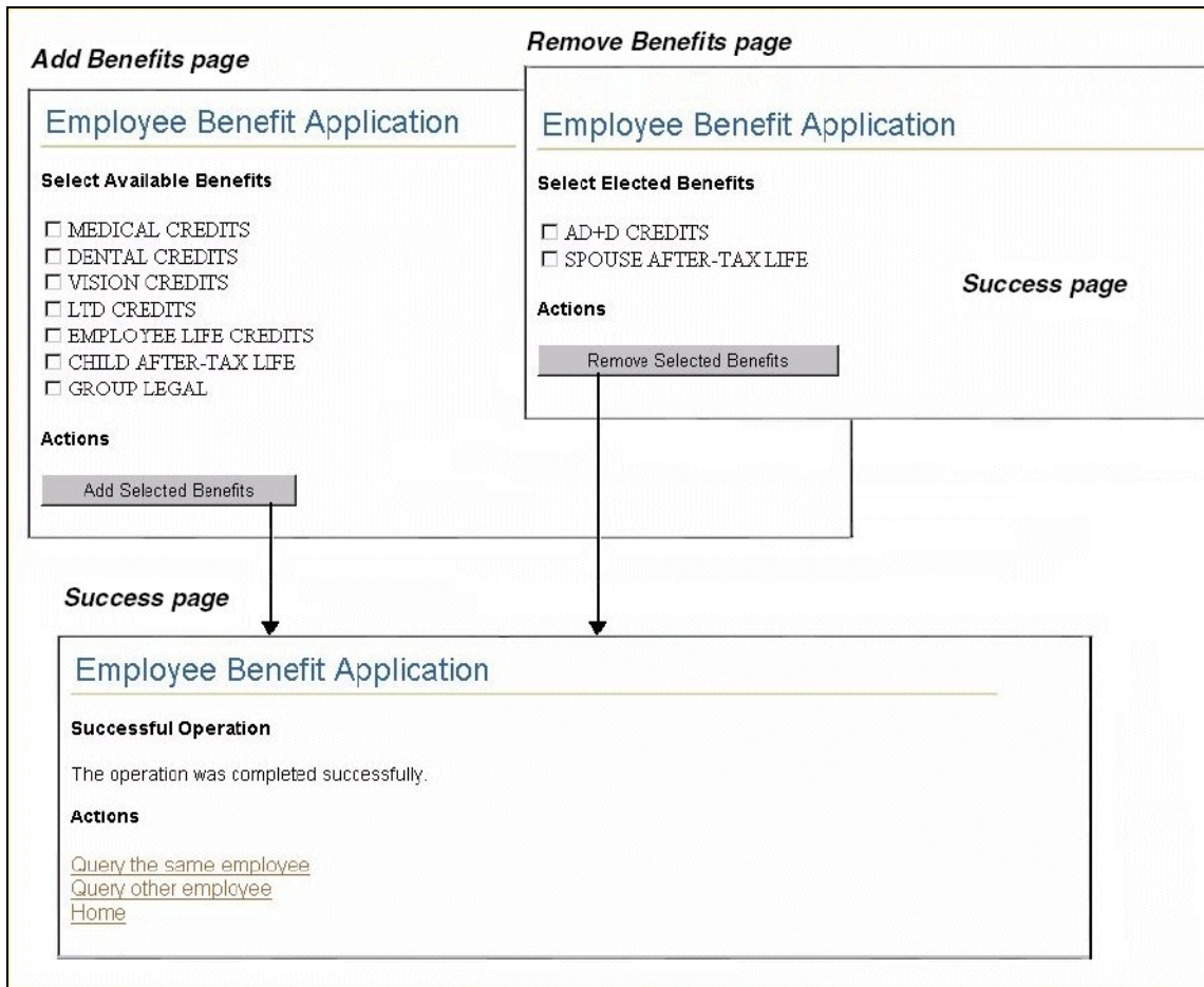
Figure 3-3 Add Benefits Page, Remove Benefits Page, and Success Page
