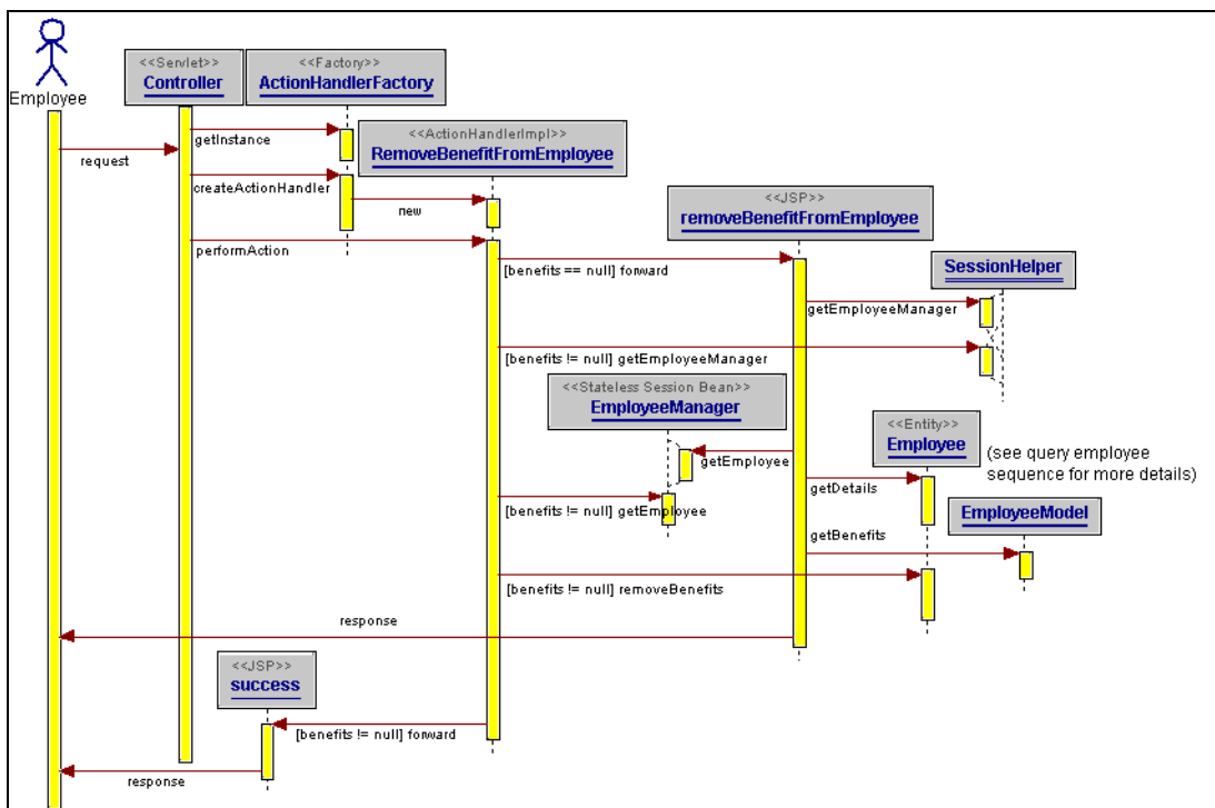
Figure 6–7 Sequence Diagram for Removing Benefits
