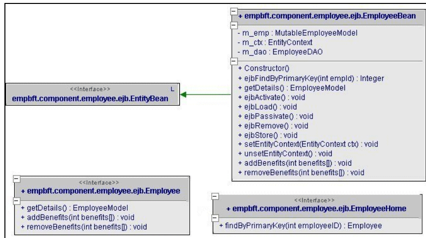
Figure 4-2 Employee Classes
