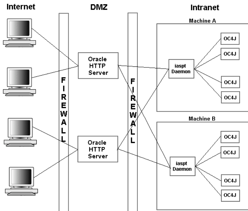
Figure 10–2 Port Tunneling
