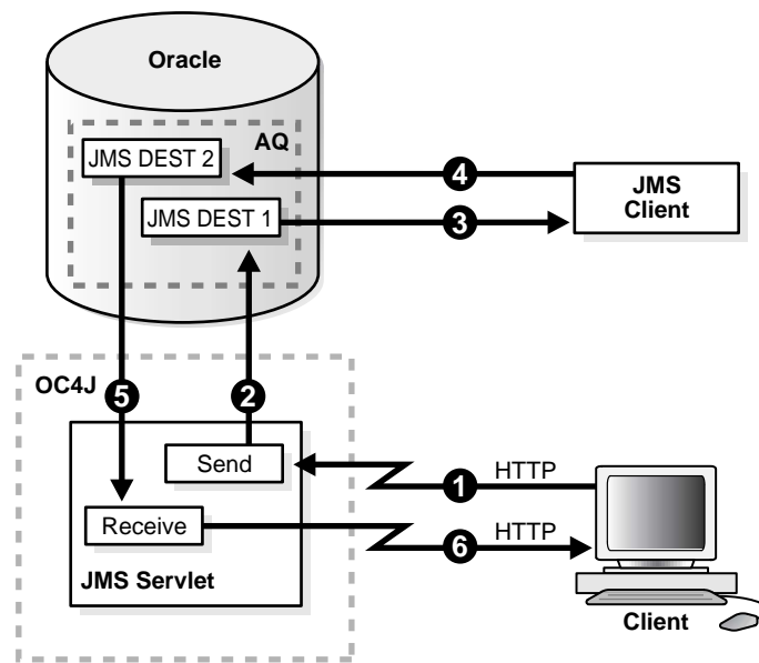
Figure 7-2 JMS Client Based JMS Web Service
