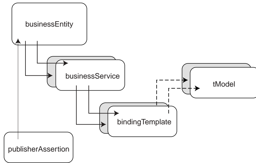
Figure 10-1 UDDI Registry Information Model
