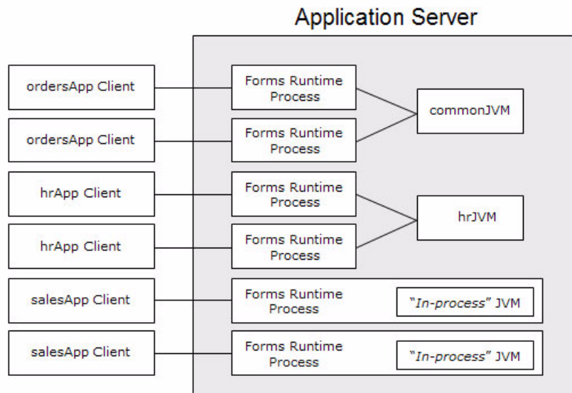
Figure 7-4 Multiple JVMs for multiple applications
