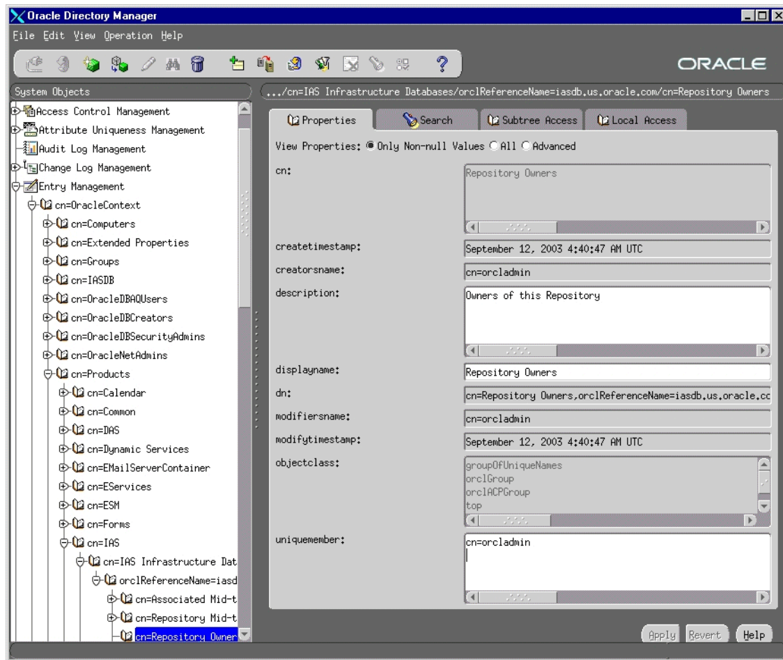
Figure 6–4 Using Oracle Directory Manager to Add Users to Metadata Repository Groups
