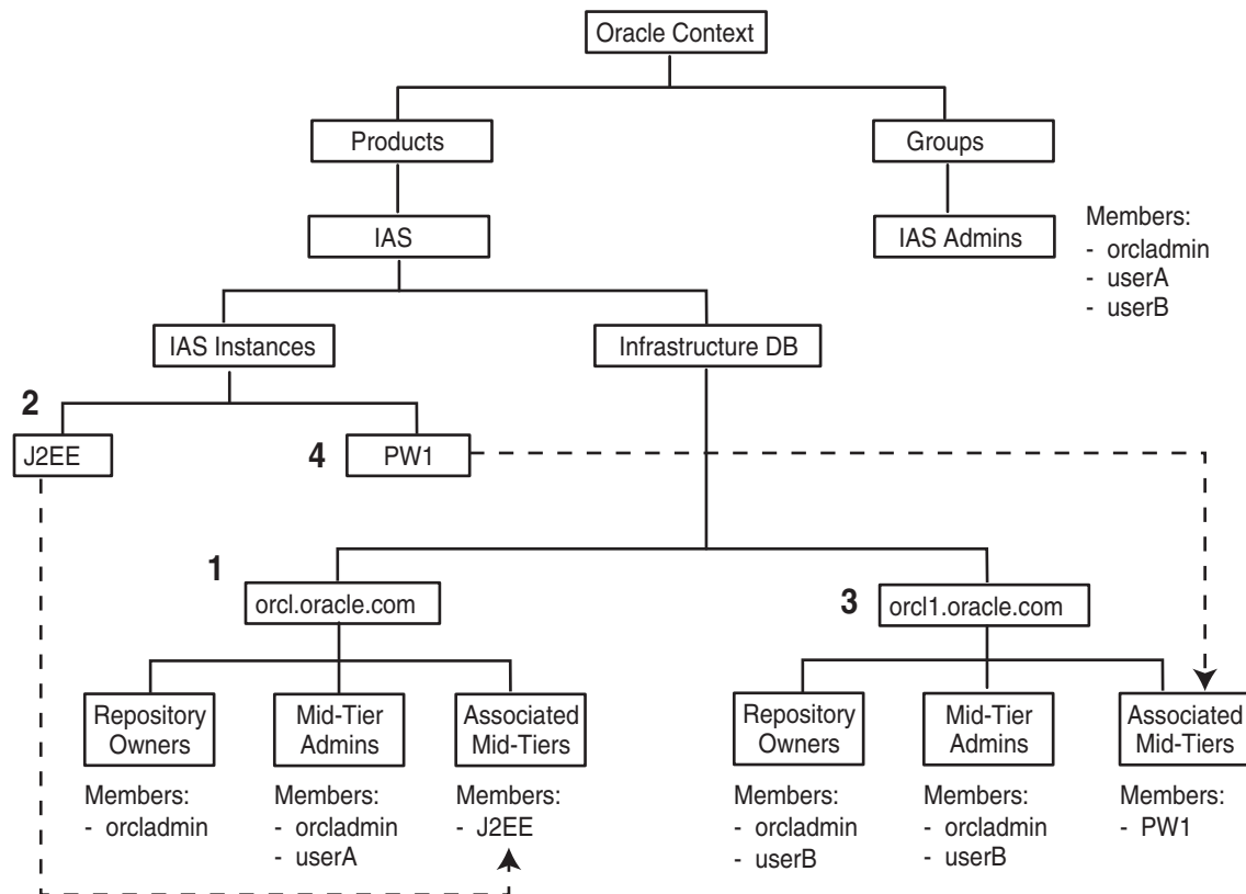
Figure 6–2 Oracle Internet Directory with Two Metadata Repositories and Two Middle Tiers
