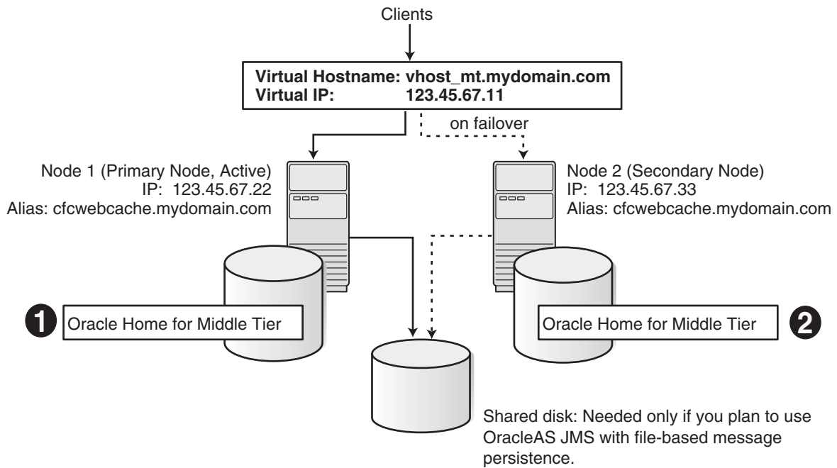
Figure 10–7 OracleAS Cold Failover Cluster (Middle-Tier) Configuration with a Single Oracle Home
