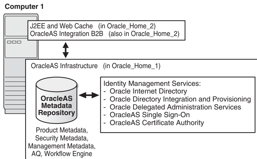
Figure 14–4 Integration B2B Topology
