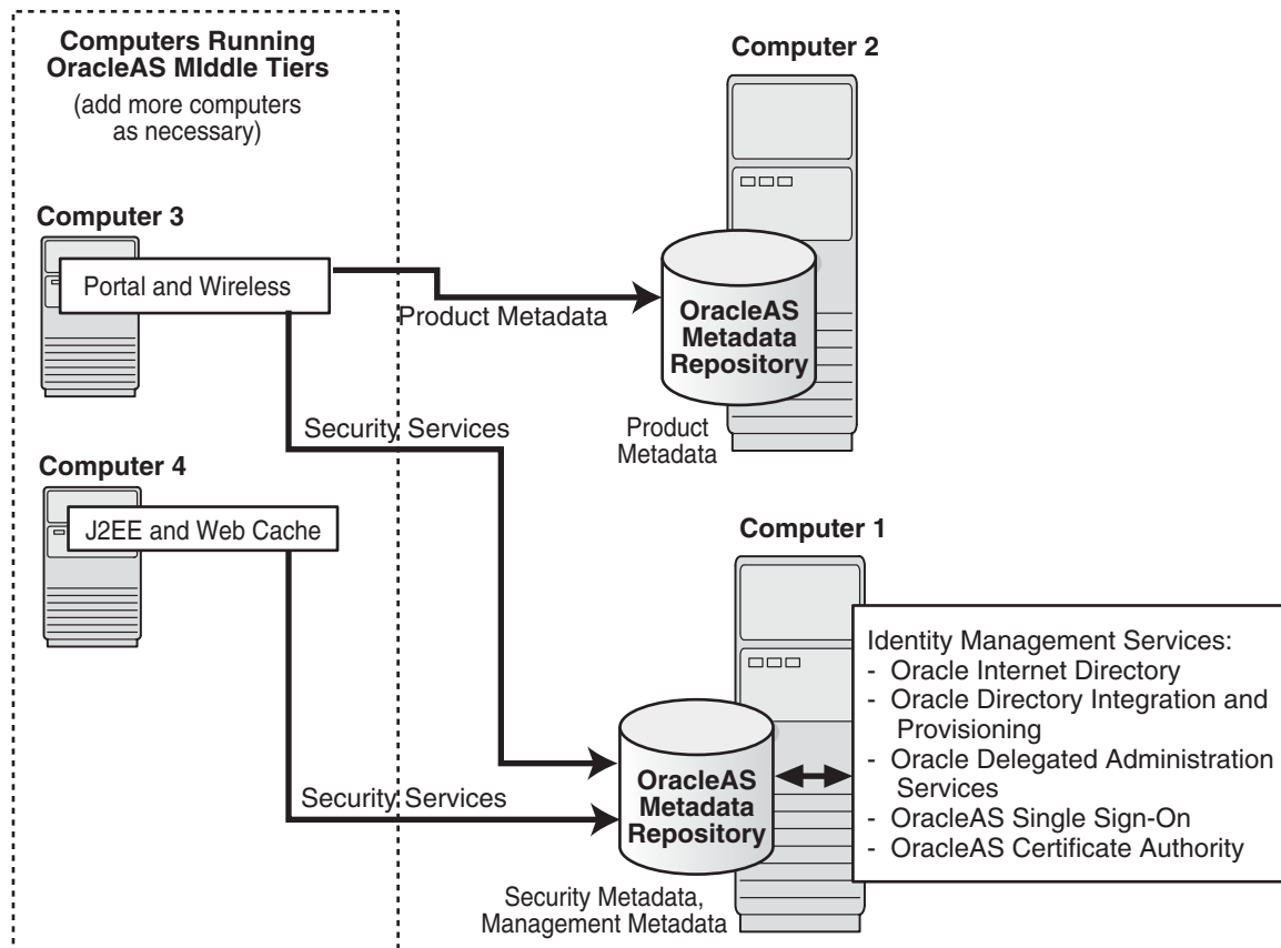
Figure 14–5 Departmental Topology
