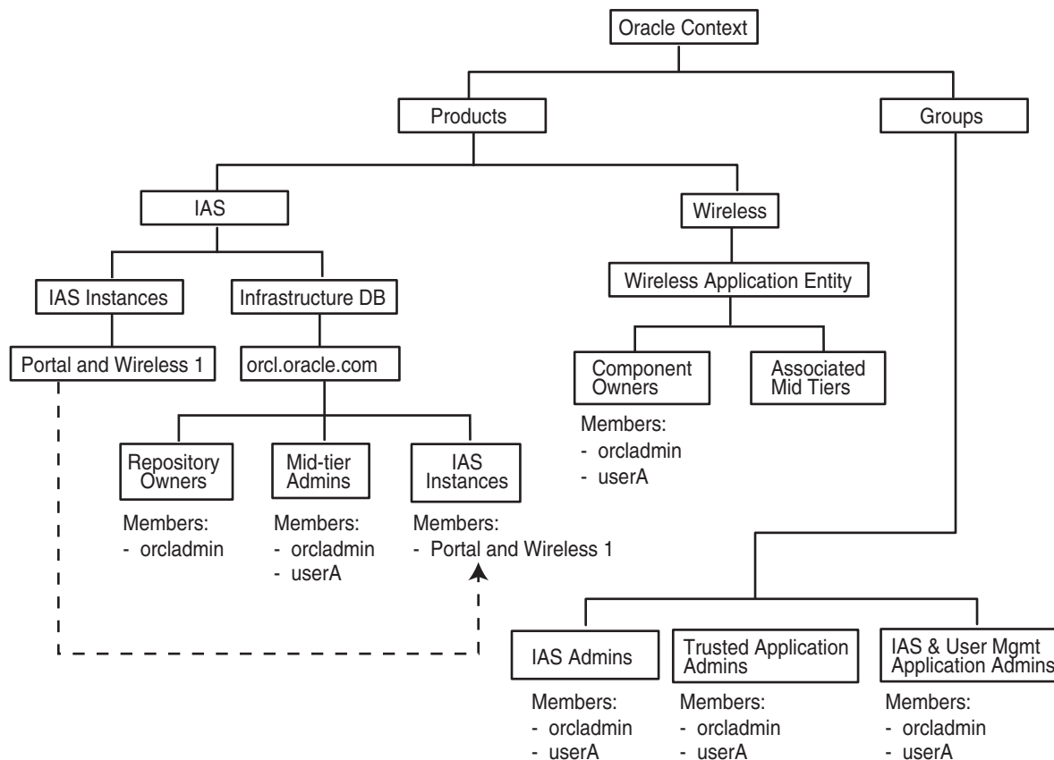
Figure 6–1 Contents of Oracle Internet Directory with One Infrastructure and One Middle Tier
