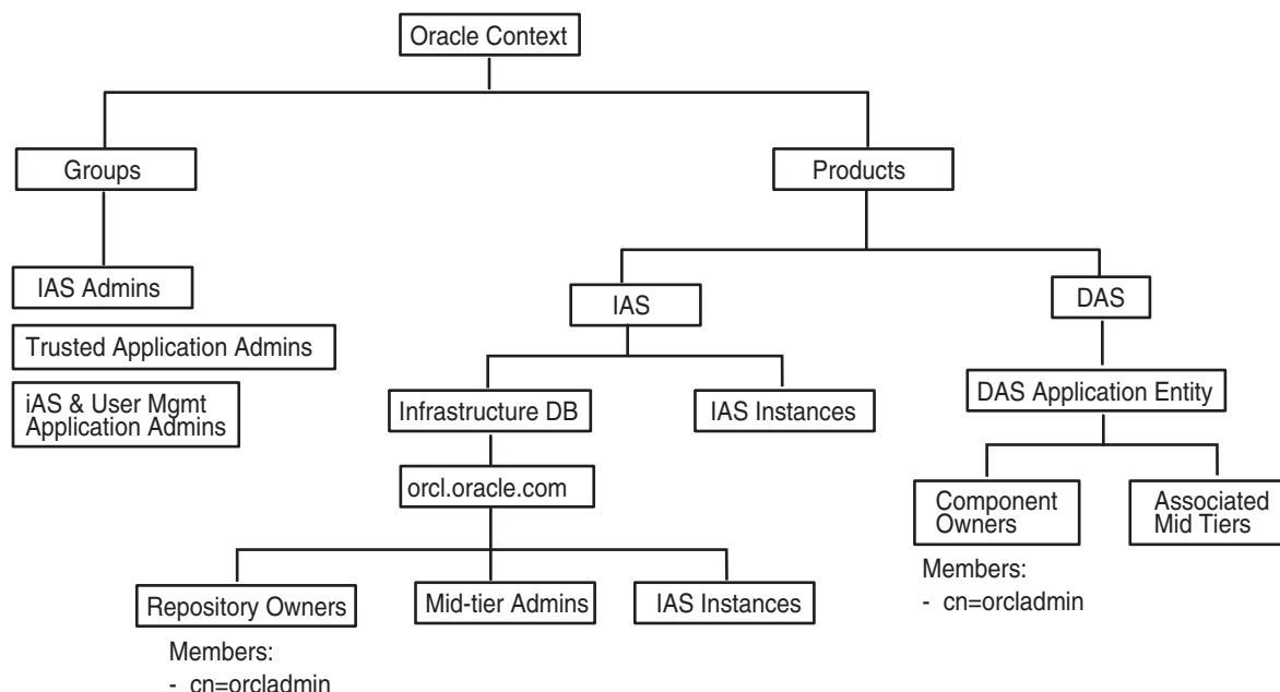
Figure 6-6 Contents of a New Oracle Internet Directory
