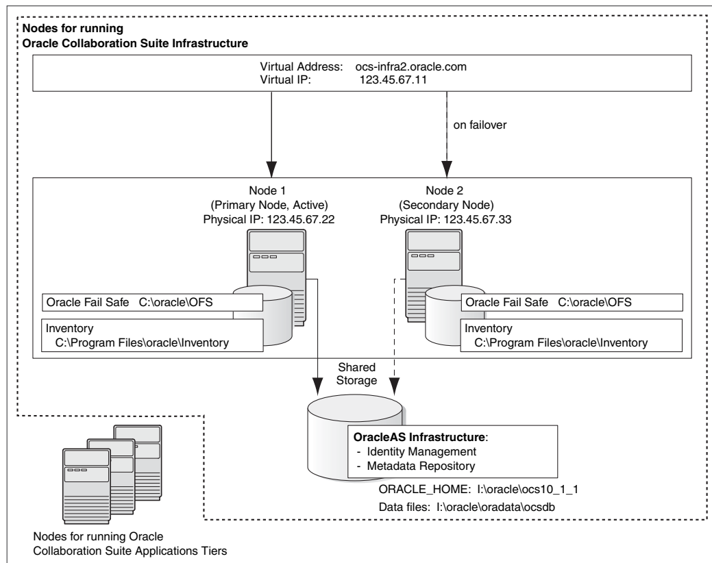
Figure 10–4 Oracle Calendar Server High Availability Configuration
