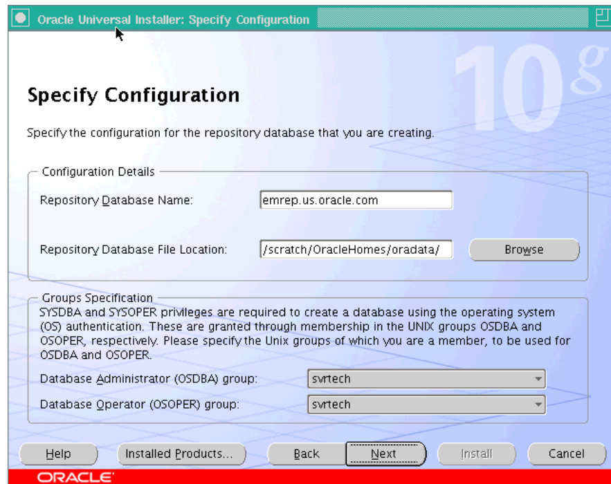
Figure 3–7 Specify Configuration
