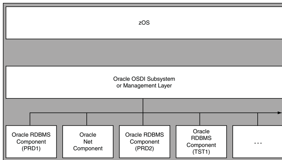
Figure 2–1 OSDI Architecture
