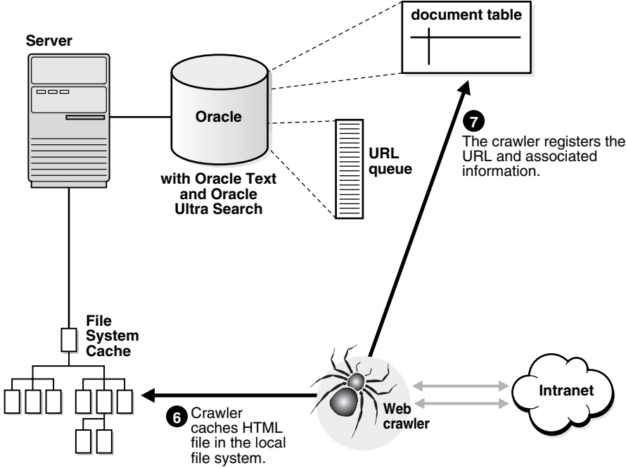
Figure 7-2 Caching URLs
