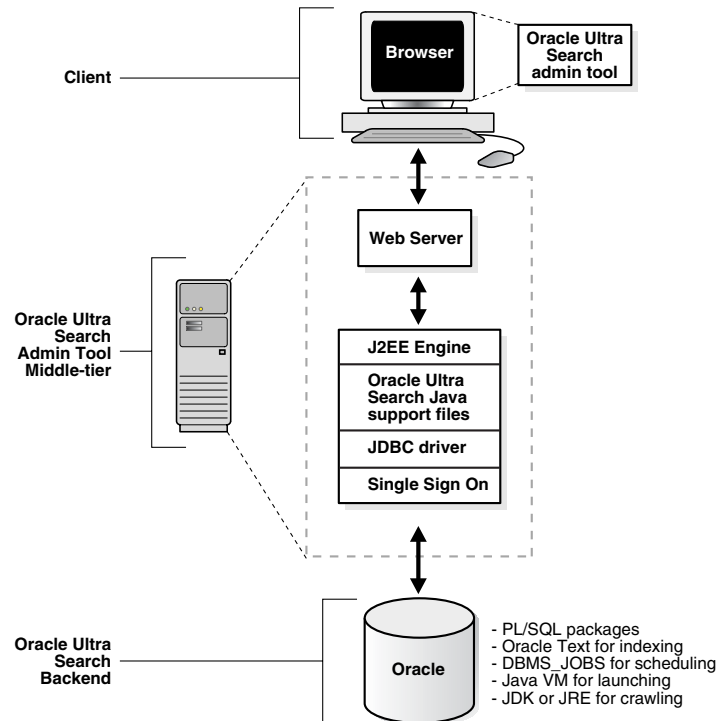
Figure 1-1 Oracle Ultra Search Architecture
