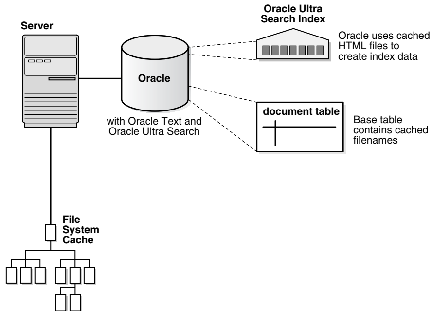
Figure 7-3 Indexing Documents
