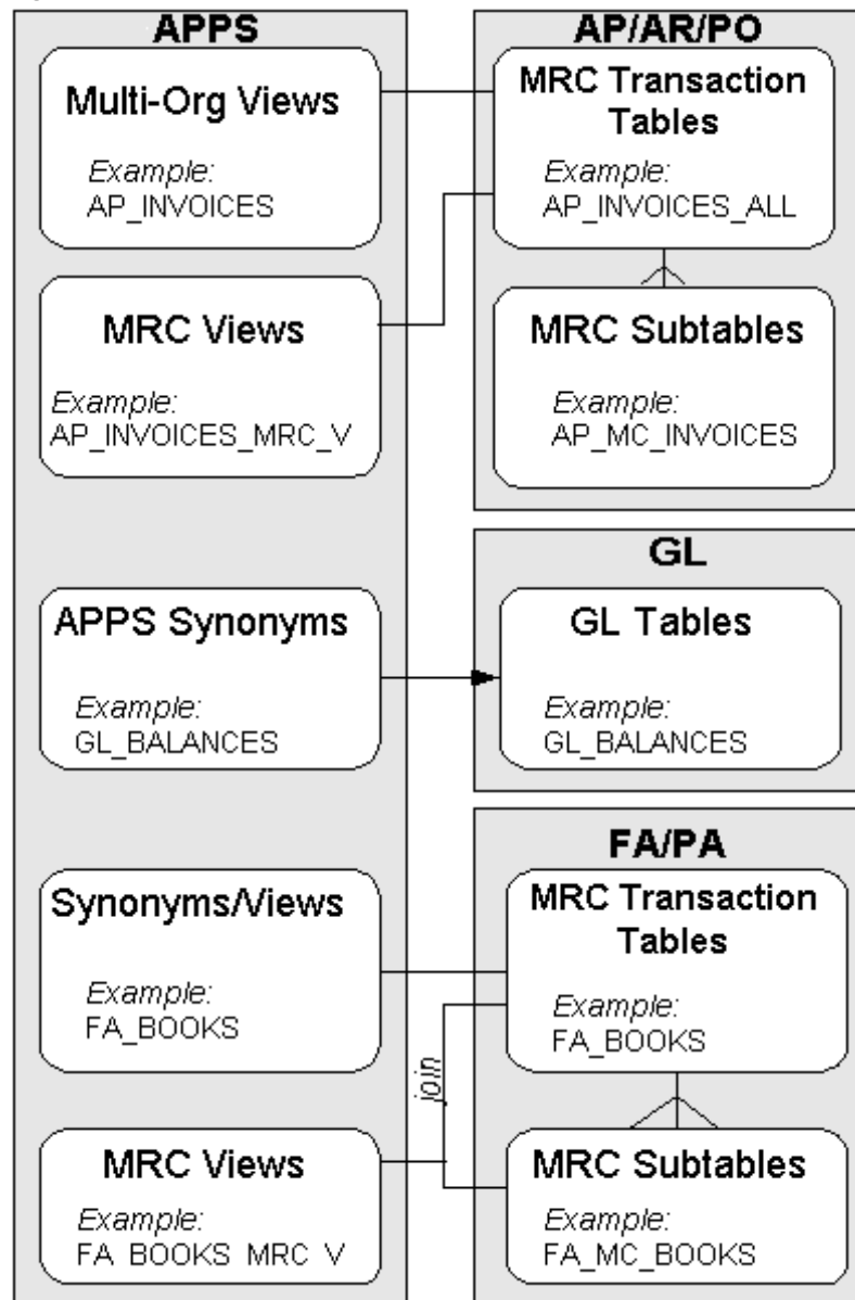
Figure 15-1 MRC Architecture
