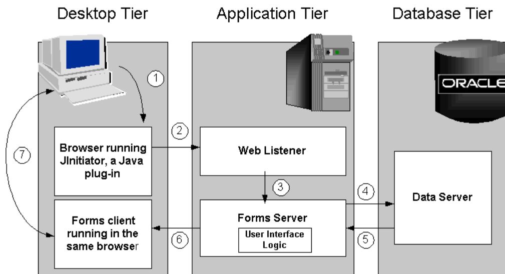
Figure 1-6 Forms Server Architecture
