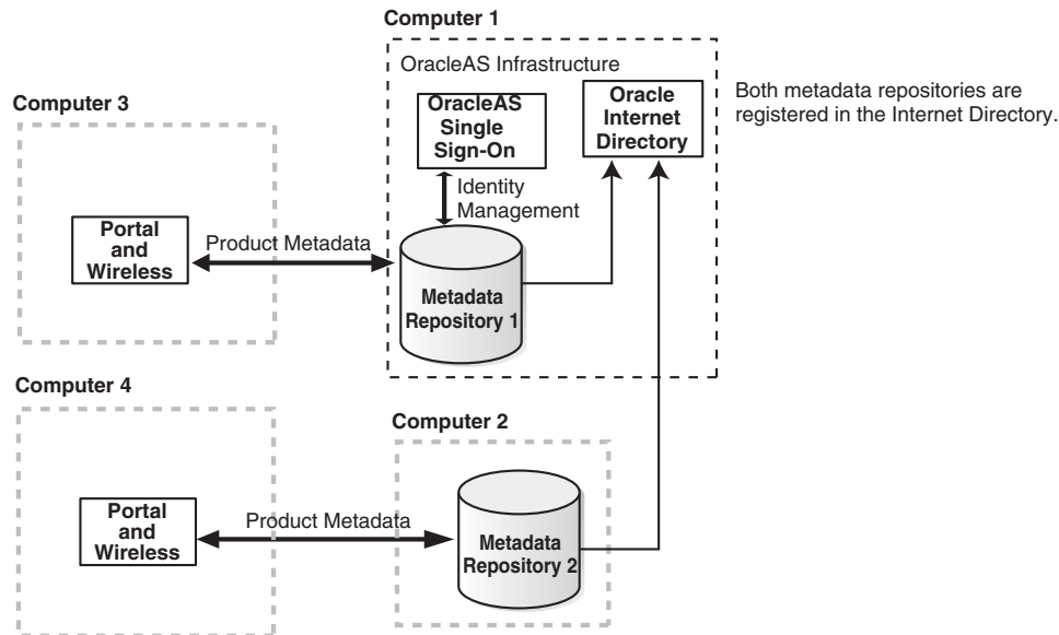
Figure 6–1 Multiple Metadata Repositories in Use
