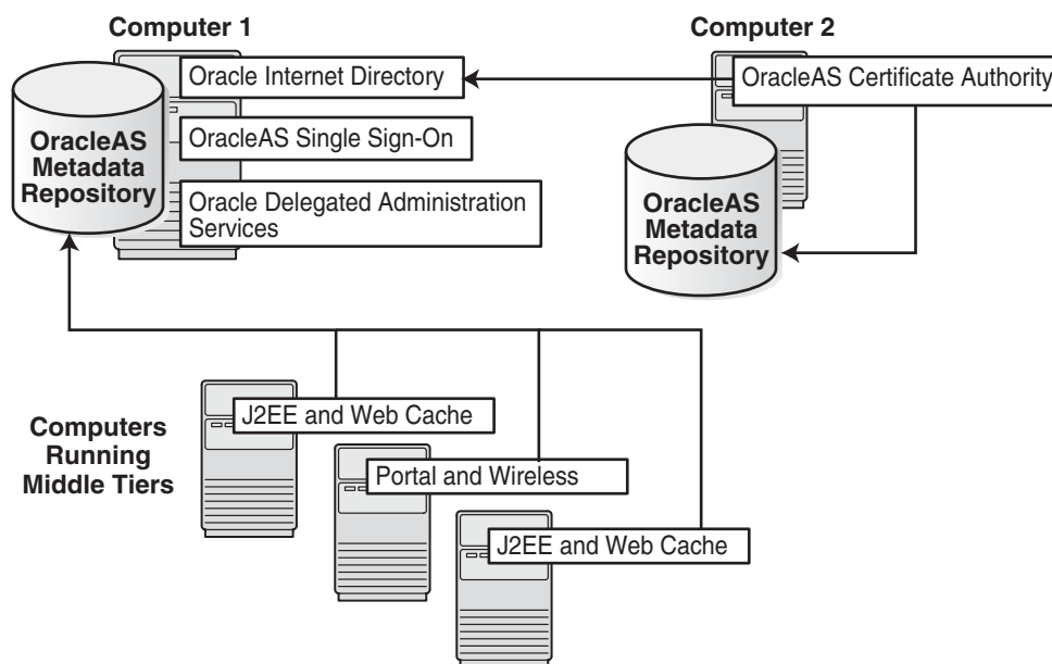
Figure 15–5 Topology for OCA
