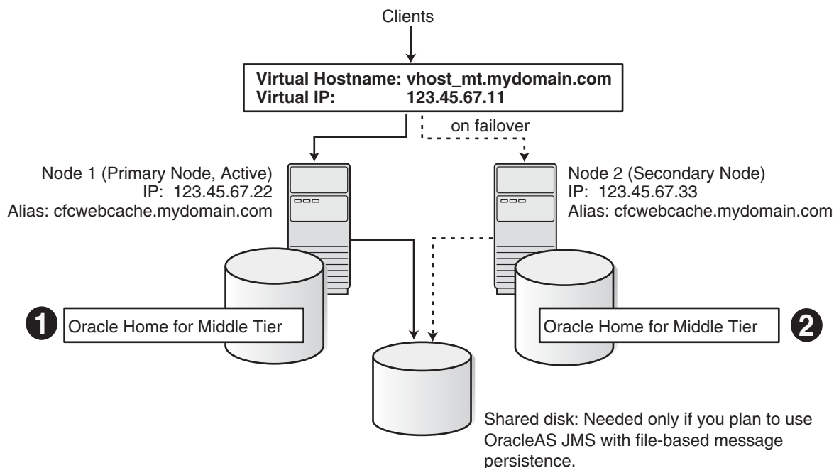
Figure 11–7 OracleAS Cold Failover Cluster (Middle-Tier) Configuration with a Single Oracle Home
