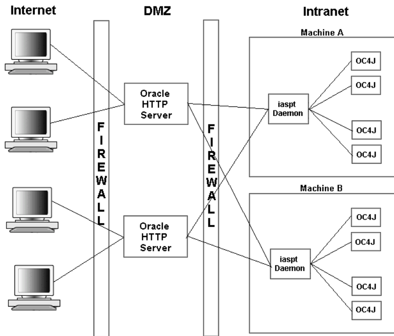
Figure 9–2 Port Tunneling
