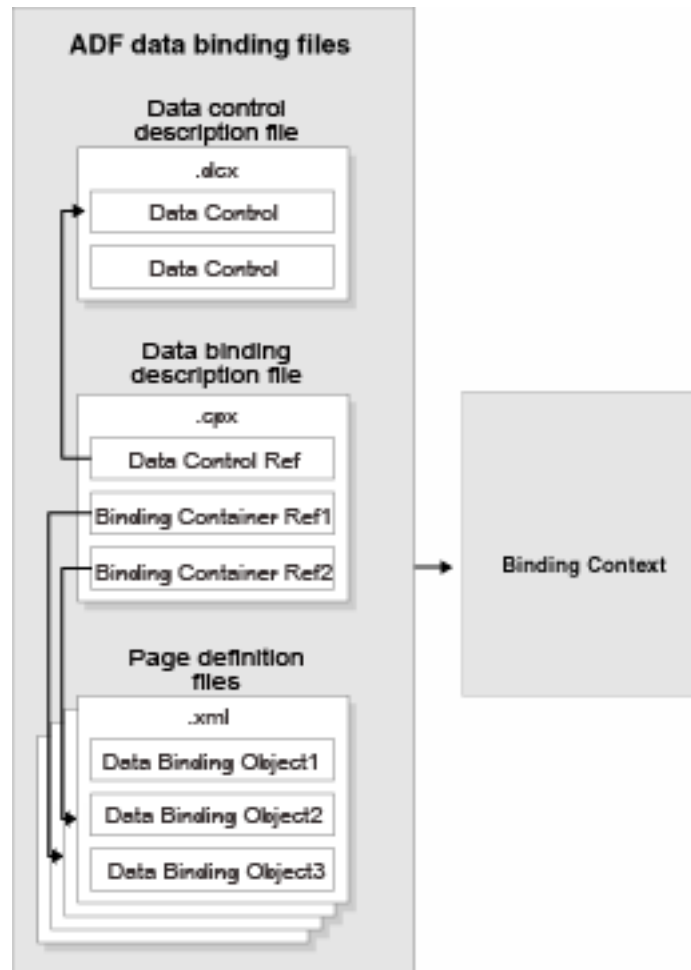
Figure 5-4 ADF Binding File Runtime Usage
