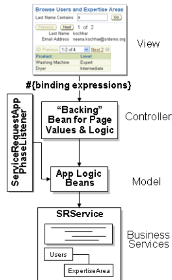
Figure 1-2 Basic Architecture of a JSF Application
