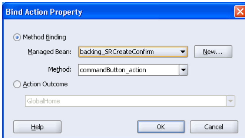
Figure 10–7 Bind Action Property Dialog for a Page with Auto-Binding Disabled
