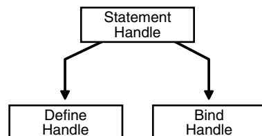
Figure 2-3 Statement Handles
