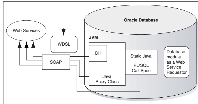
Figure 12–2 Calling Web Services From Within the Database
