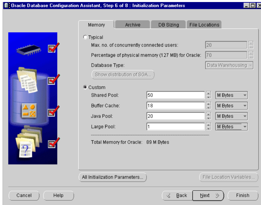
Figure 9–1 Configuring Oracle JVM Memory Parameters
