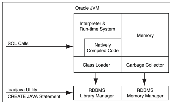
Figure 1–8 Main Components of Oracle JVM
