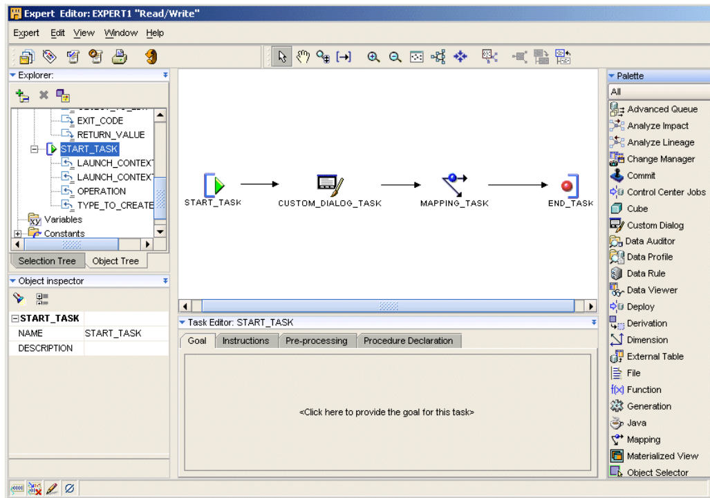
Figure 4–2 Expert Editor
