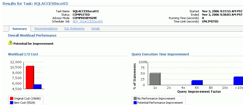
Figure 11–3 Suggested Improvements
