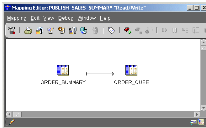
Figure 6–4 Publish_Sales_Summary Mapping
