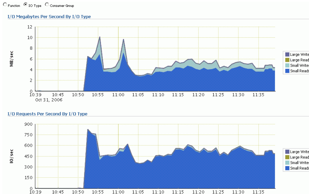
Figure 11–2 Monitoring I/O
