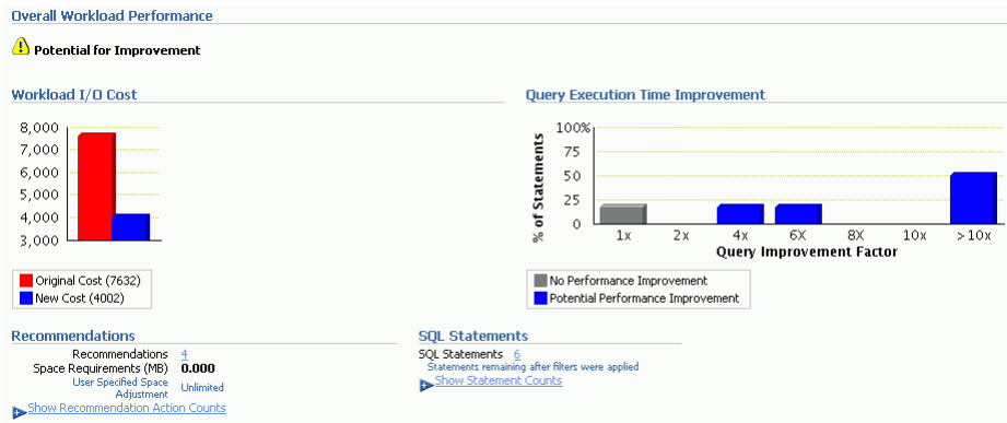
Figure 12–3 Partitioning Results
