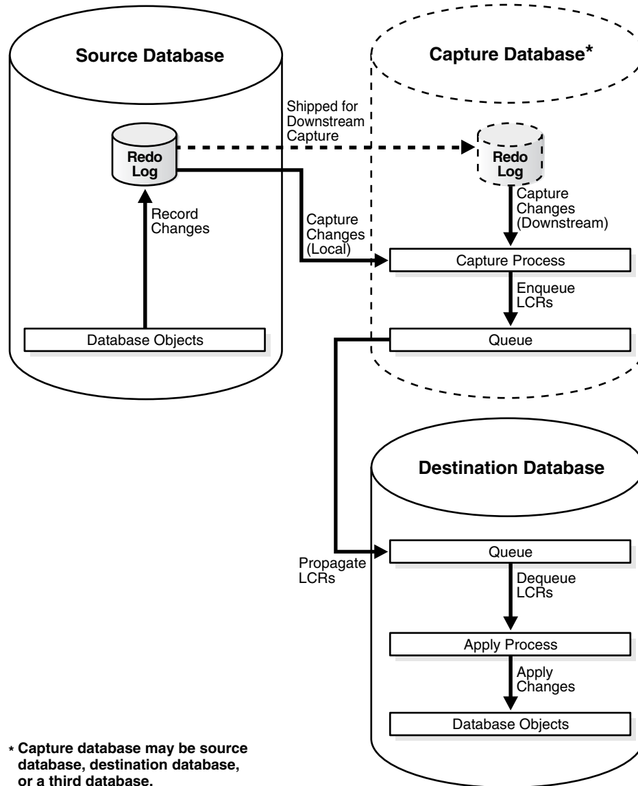
Figure D-1 Online Database Upgrade with Oracle Streams
