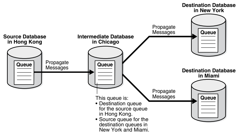
Figure 3-4 Example Directed Networks Environment
