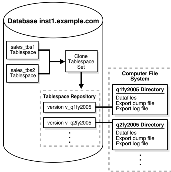
Figure 30-1 Example Tablespace Repository
