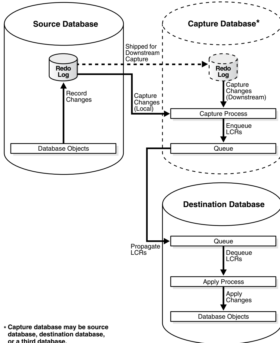
Figure E-1 Online Database Maintenance with Oracle Streams
