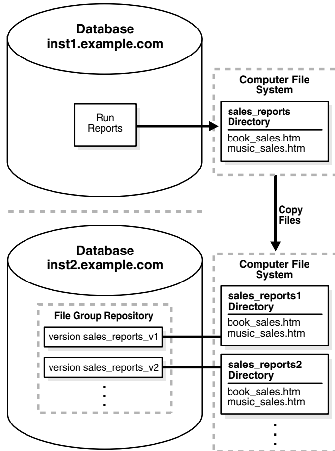
Figure 30-5 Example File Group Repository
