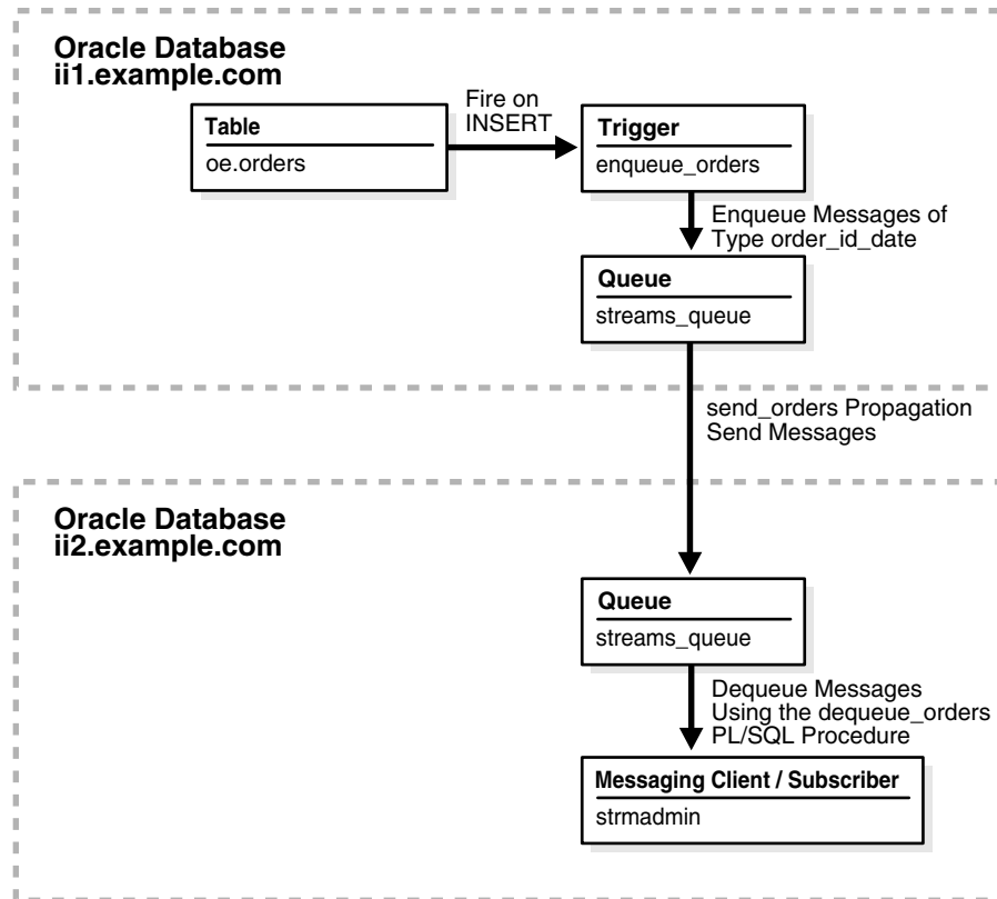
Figure 1–7 Sample Messaging Configuration
