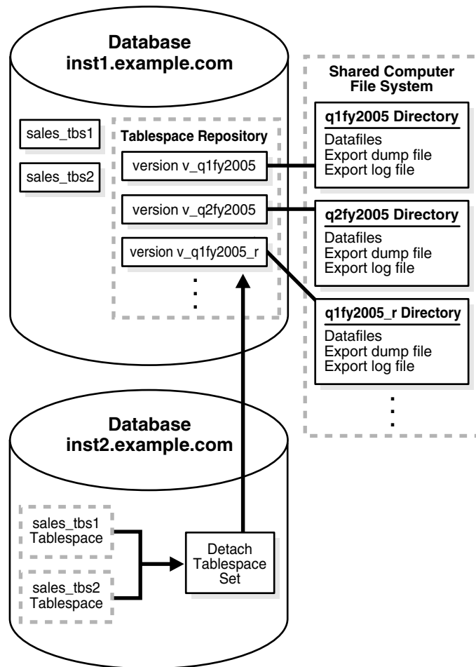
Figure 30-3 Detaching Tablespaces with a Shared File System
