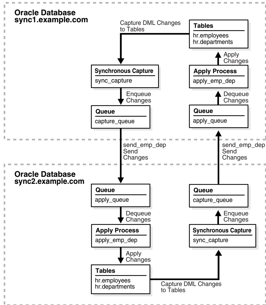
Figure 1–4 Sample Replication Configuration With Synchronous Captures
