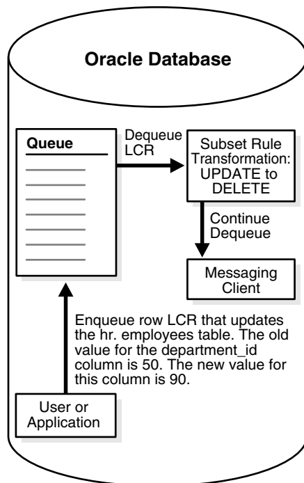
Figure 6–5 Row Migration During Dequeue by a Messaging Client
