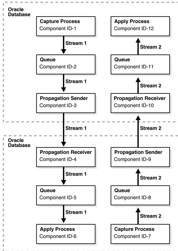
Figure 22–1 Oracle Streams Topology with Two Separate Stream Paths
