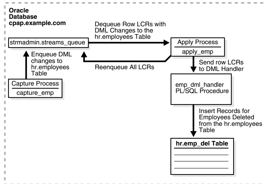
Figure 1–6 Sample Single Database Capture and Apply Configuration
