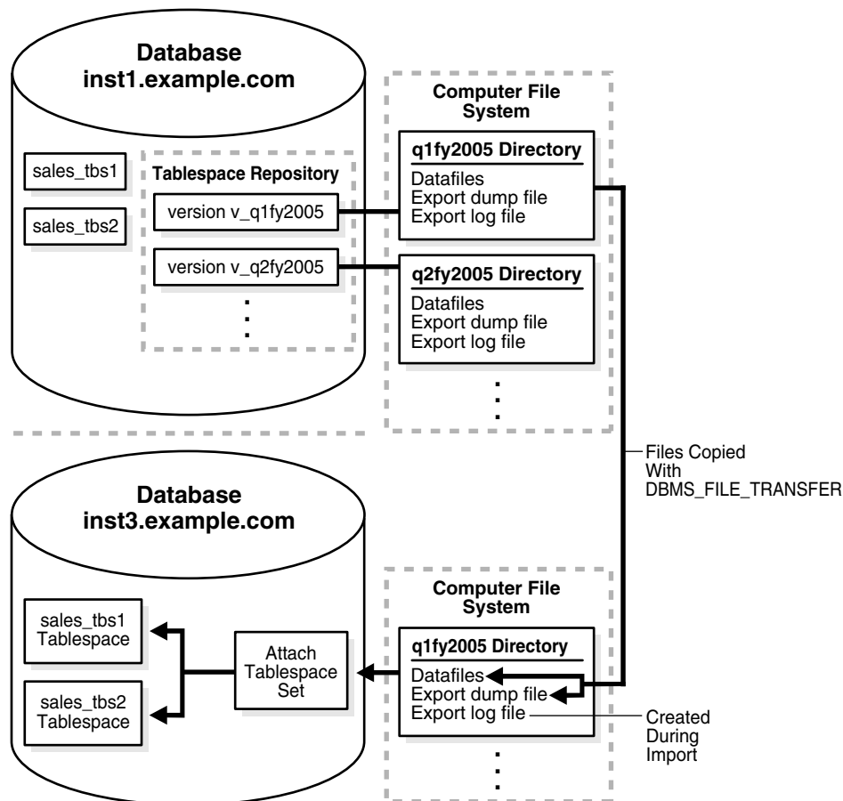
Figure 30-4 Attaching Tablespaces Without a Shared File System
