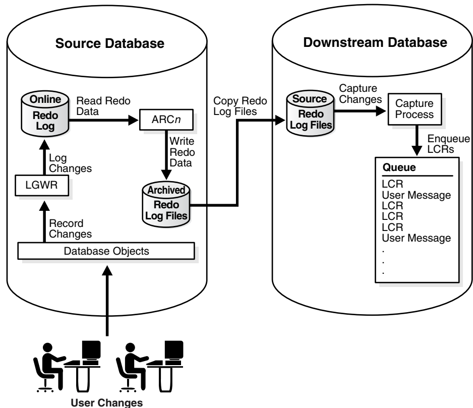
Figure 2-3 Archived-Log Downstream Capture
