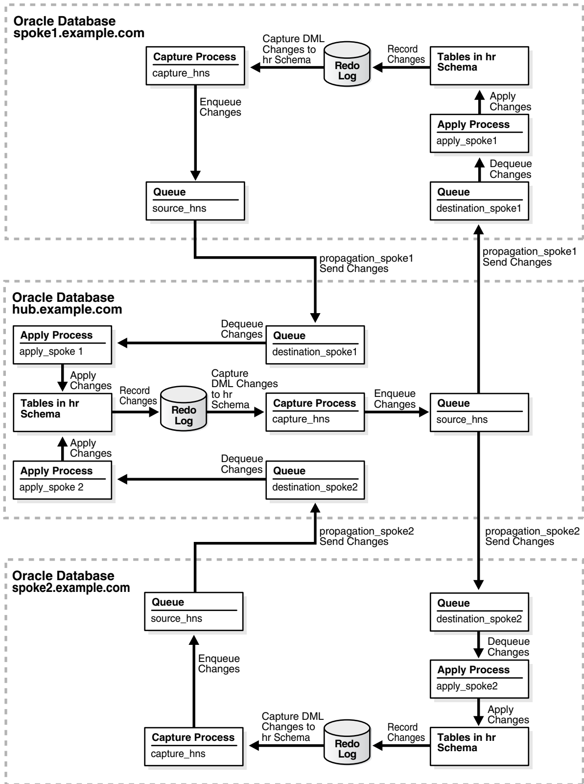
Figure 1-2 Sample Hub-and-Spoke Replication Configuration
