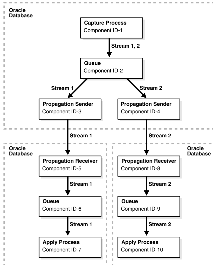
Figure 22–2 Oracle Streams Topology with Multiple Apply Processes for a Single Source
