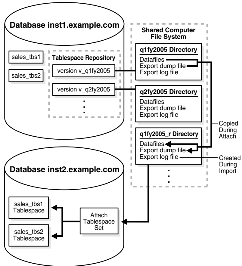
Figure 30–2 Attaching Tablespaces with a Shared File System
