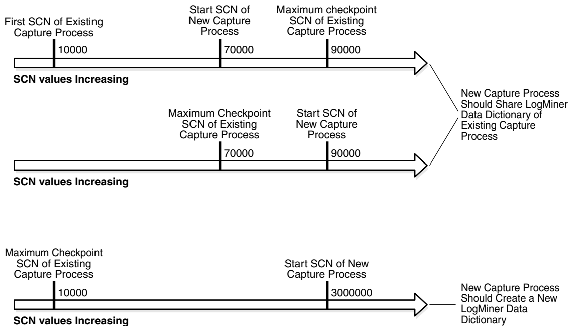
Figure 2–7 Deciding Whether to Share a LogMiner Data Dictionary
