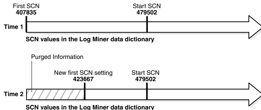
Figure 2–5 Start SCN Higher than Reset First SCN
