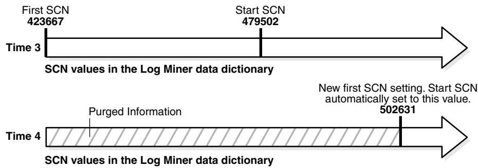
Figure 2-6 Start SCN Lower than Reset First SCN
