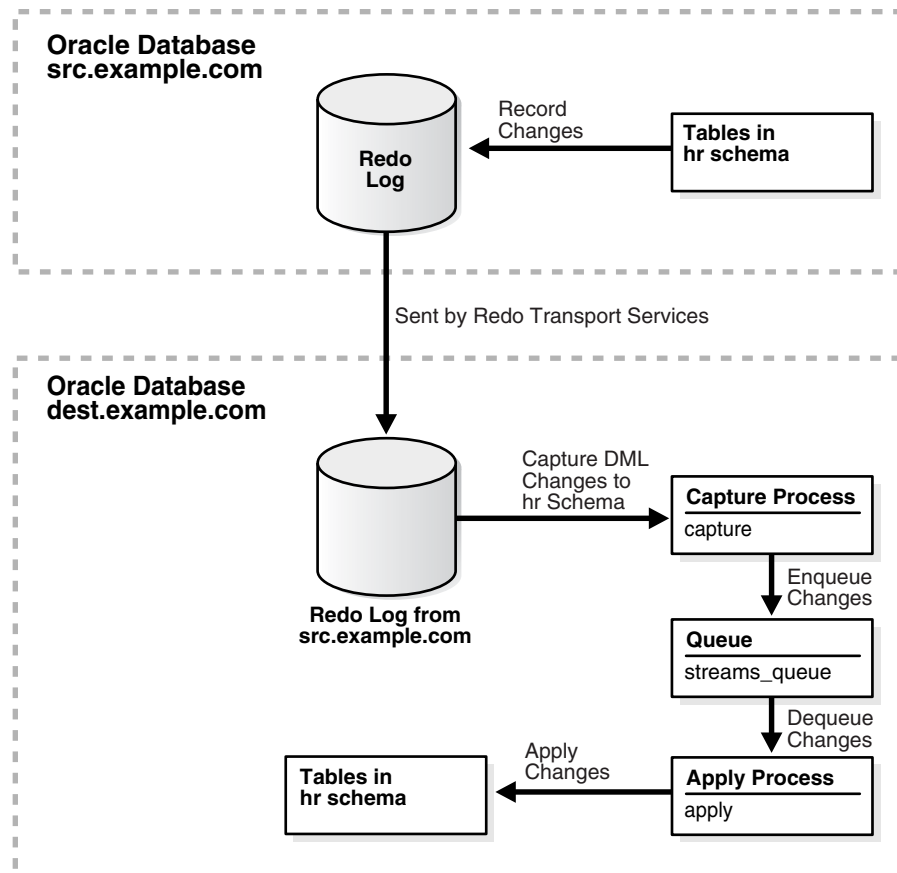
Figure 1–3 Sample Replication Configuration With Downstream Capture
