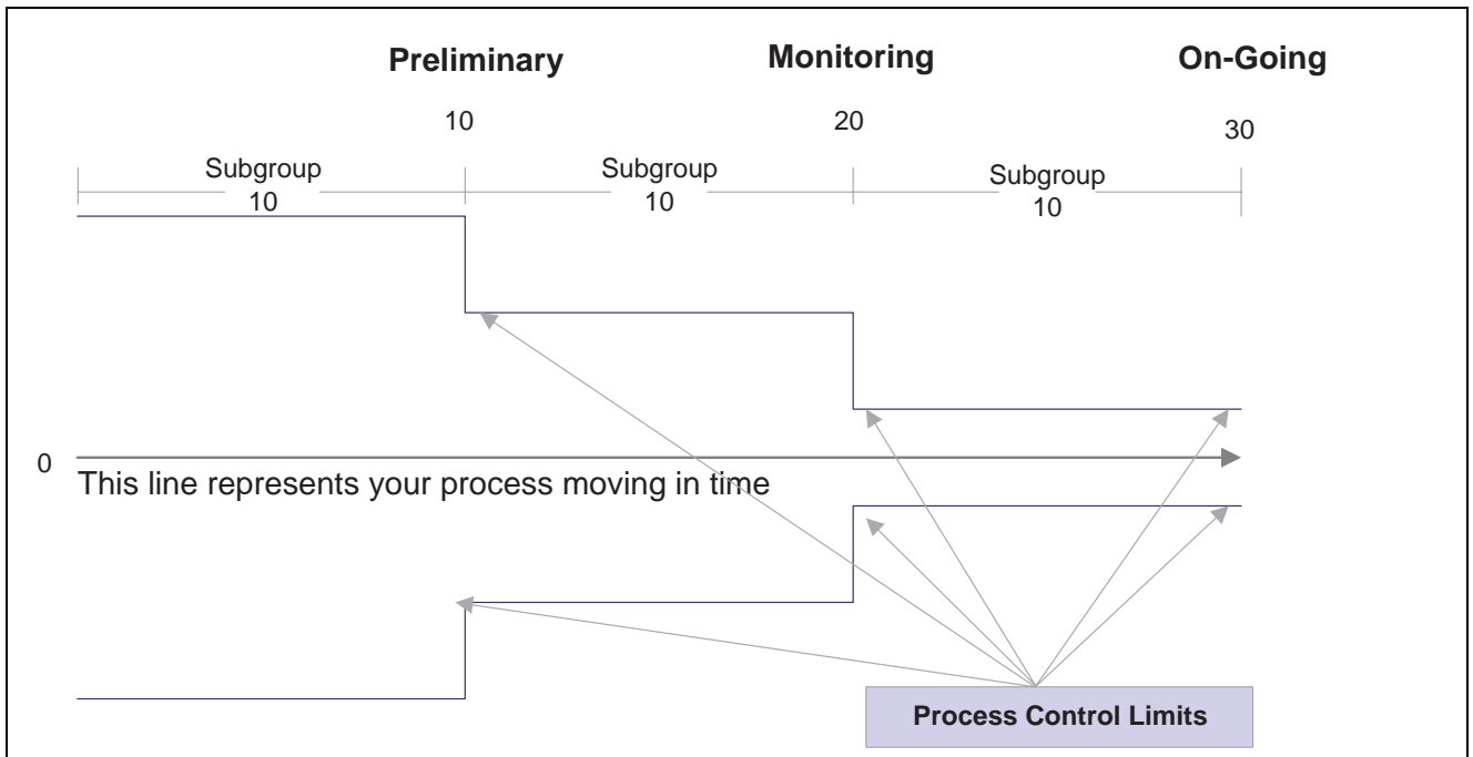
Understanding process control limits
