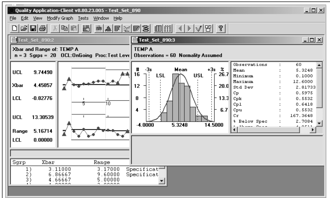
Example of graph-display layout
