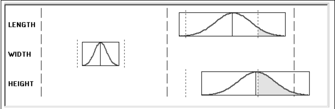
Overlaying distribution curves on box plots
