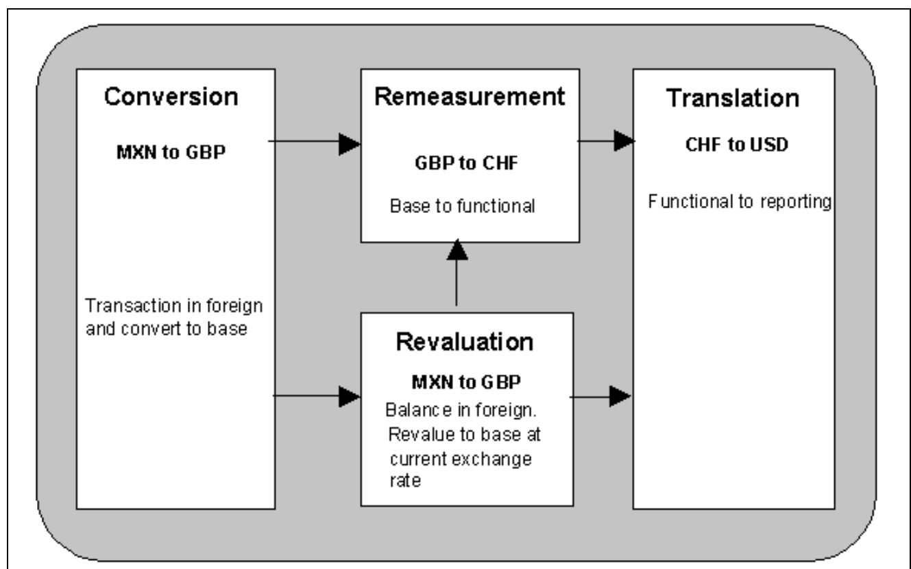
Multicurrency Calculations
