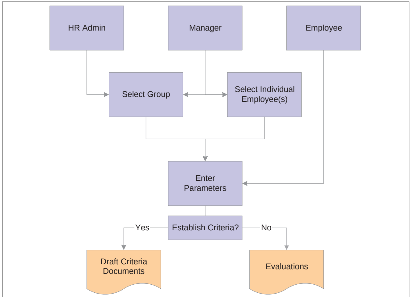
Document generation processes
