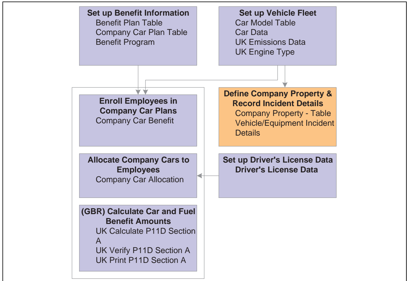
Administer Company Cars business process
