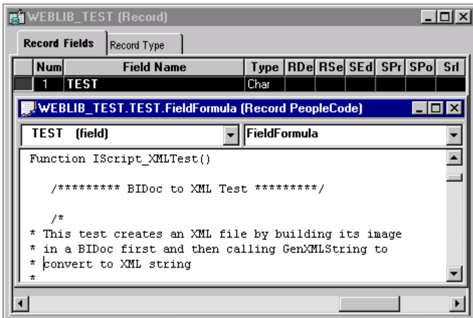
IScript Function in Test Field: Field Formula
