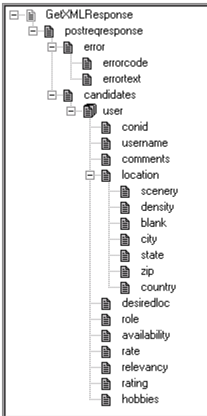
Transaction Outputs: XML Response
