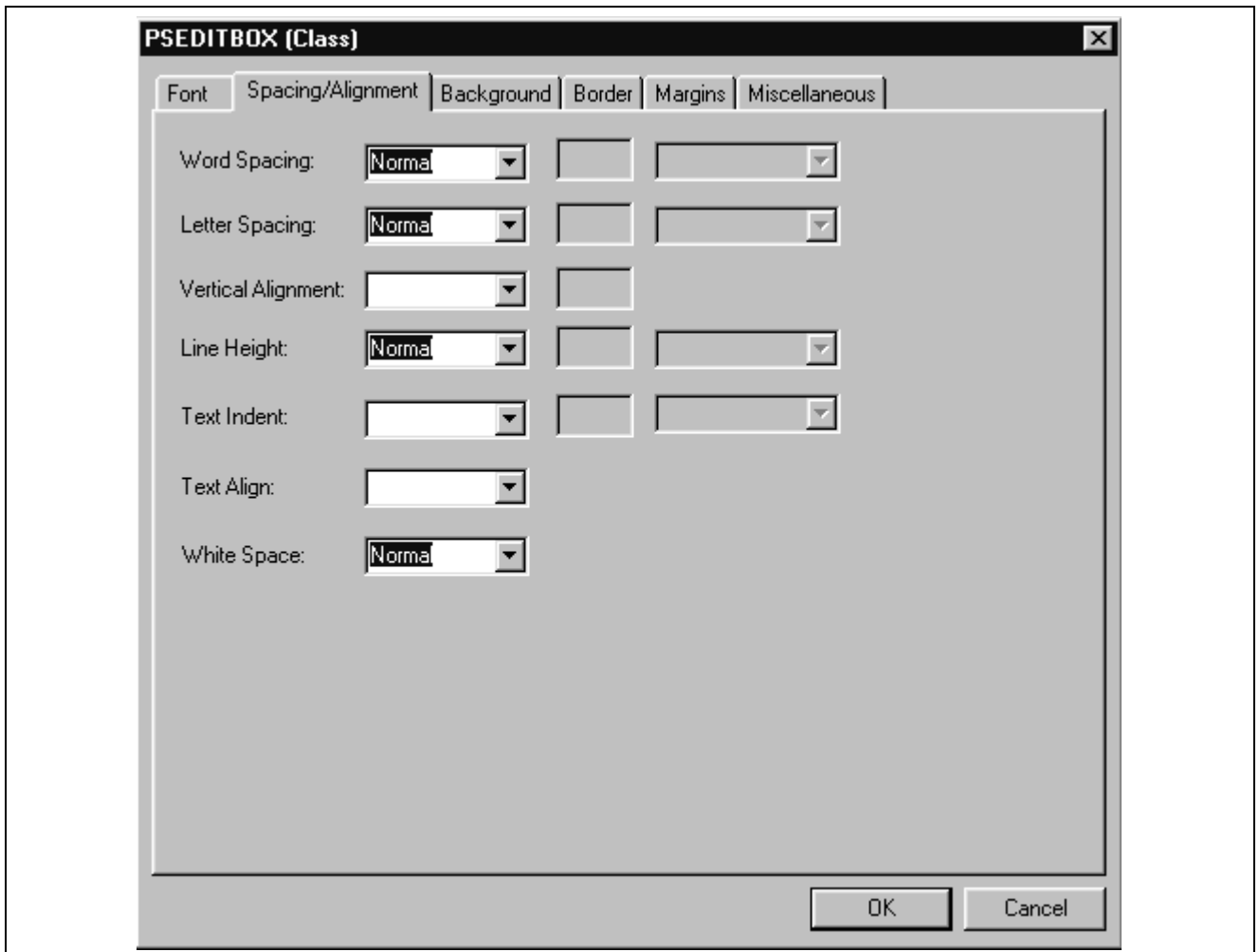
PSEDITBOX (Class) dialog box: Spacing/Alignment tab
