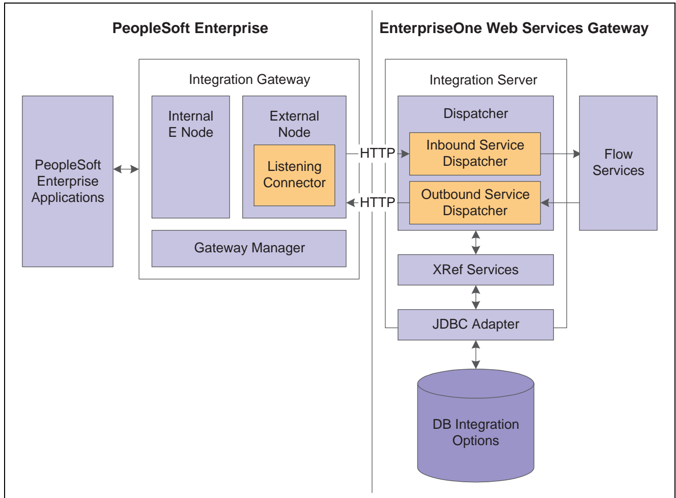
PeopleSoft EnterpriseOne WSG Dispatcher and PeopleSoft Enterprise Integration Gateway communications architecture
