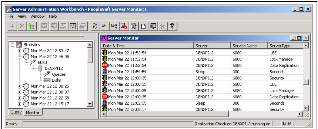
SAW Server Monitor window
