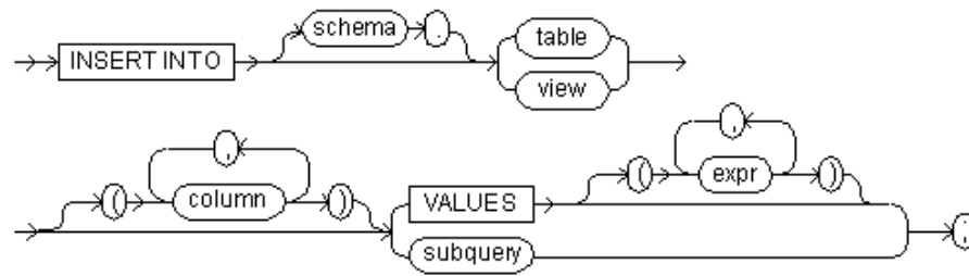
Figure 4–47 The INSERT Command
