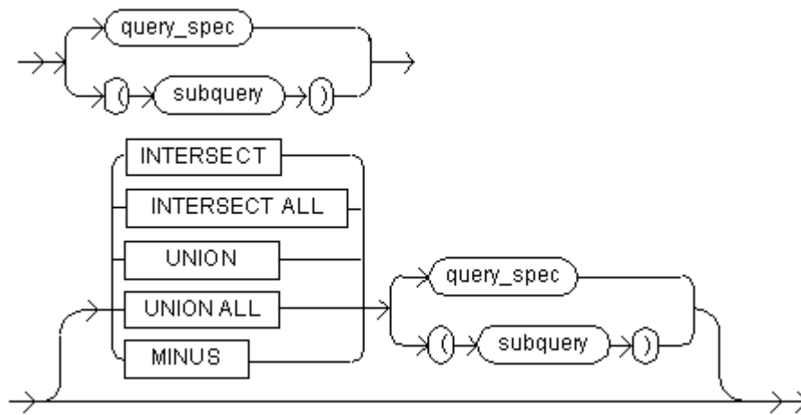
Figure 4-52 The subquery Expression
