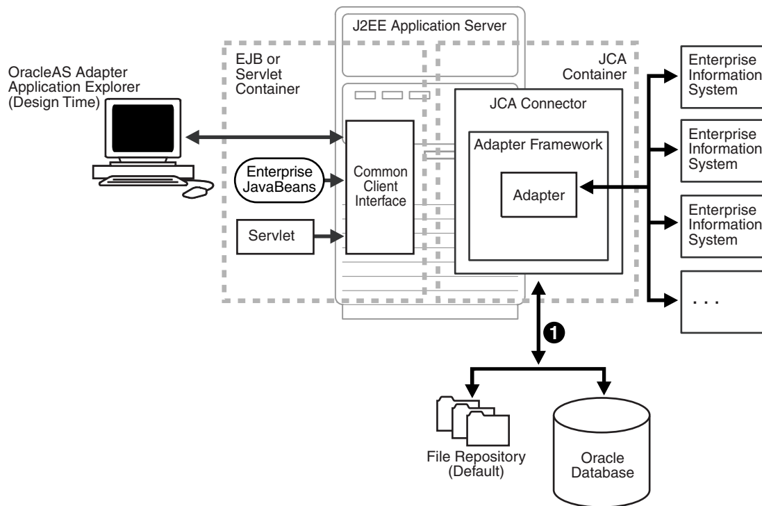
Figure 1–2 Oracle Application Server Adapter J2CA Generic Architecture
