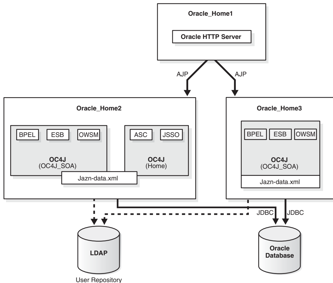
Figure 1–8 Cluster with Multiple SOA Middle Tiers and a Remote Oracle HTTP Server
