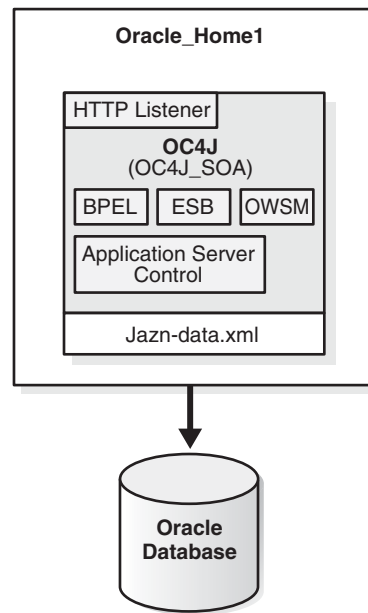
Figure 1–4 J2EE Server with the SOA Suite
