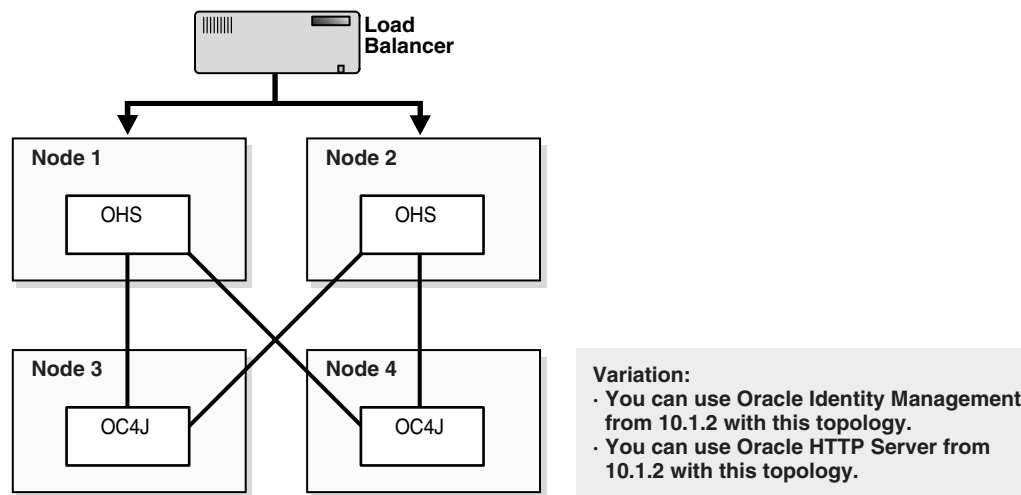
Figure 6–2 Active-Active Topology with Oracle HTTP Server and OC4J in Separate Oracle Homes
