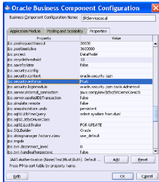
Figure 30–5 ADF BC Configuration Dialog, Properties Panel
