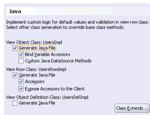
Figure 5–30 View Object Custom Java Generation Options
