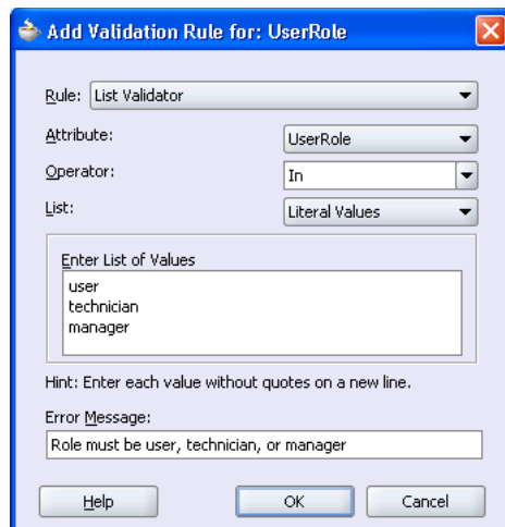
Figure 2–9 The List Validator Ensures That UserRole Has One of Three Legal Values
