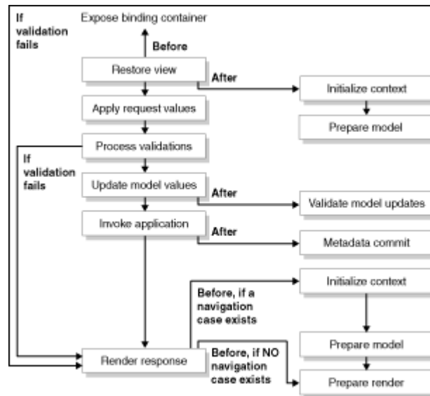
Figure 13–2 The Lifecycle of a Page Request in an ADF Application Using ADF Faces Components
