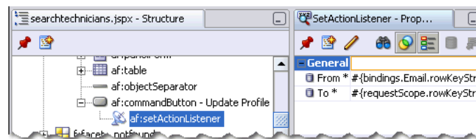
Figure 2–34 Declaratively Setting a Request Attribute
