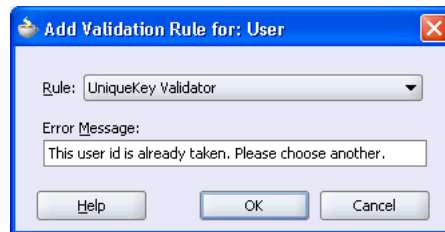
Figure 2-7 Adding a New UniqueKey Validator
