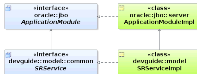
Figure 8–6 Custom Service Interface Extends the Base ApplicationModule Interface
