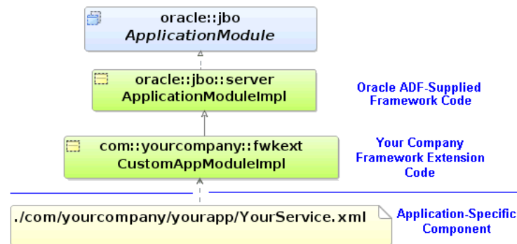
Figure 25–3 XML-Only Component Reference an Extended Framework Base Class
