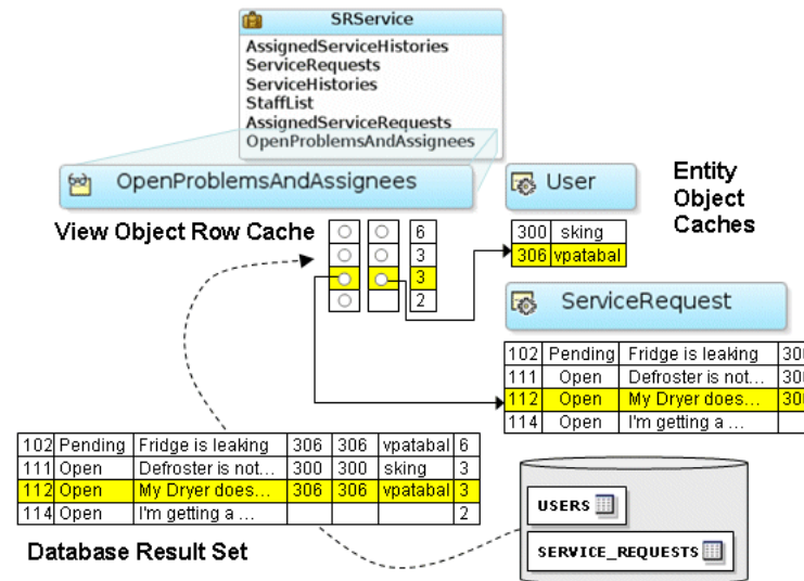
Figure 7–24 View Rows Are Partitioned into Entity Rows in Entity Caches
