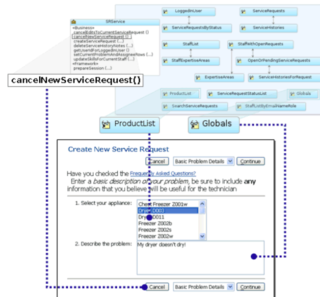
Figure 10–23 Service Method and View Objects for the SRCreate Page
