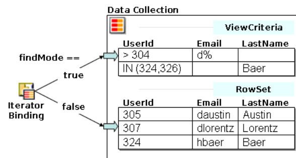
Figure 10–11 When Find Mode is True, Iterator Binding Points at ViewCriteria Row Set Instead
