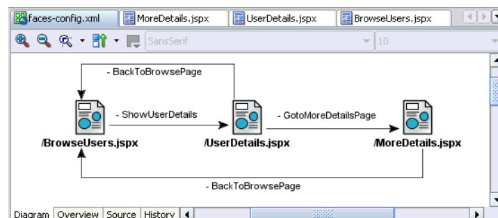
Figure 1–5 Visualizing JSF Navigation Rules in JDeveloper's Page Flow Diagram
