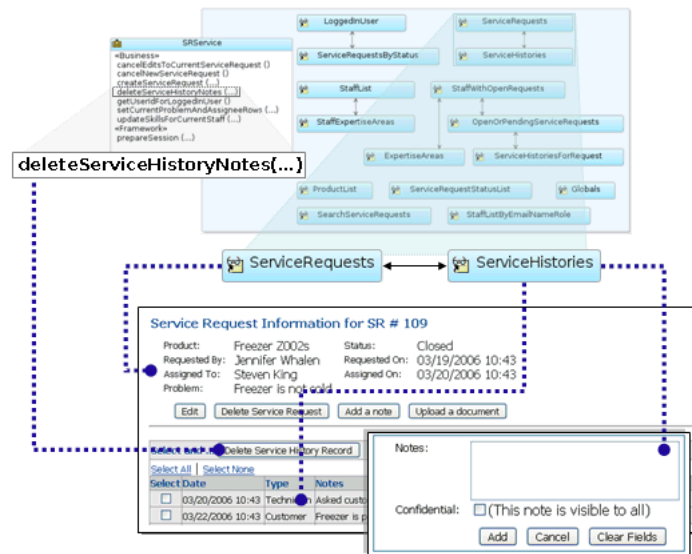
Figure 10-17 Service Method and View Objects for the SRManage Page
