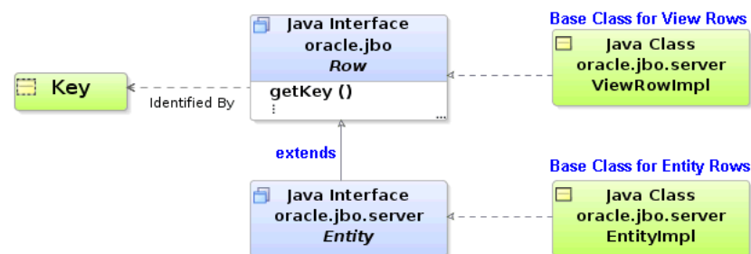
Figure 7-21 Any View Row or Entity Row Supports Retrieving Its Identifying Key
