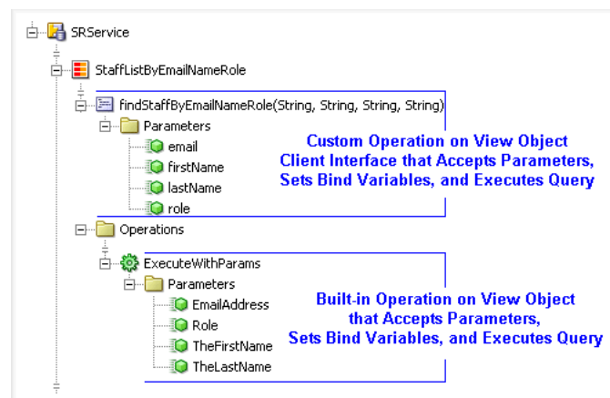
Figure 10–9 Work with Named Bind Variables Using Either a Built-in or Custom Operation
