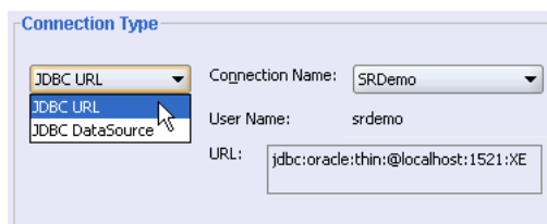
Figure 8–2 Connection Type Setting in Configuration Editor
