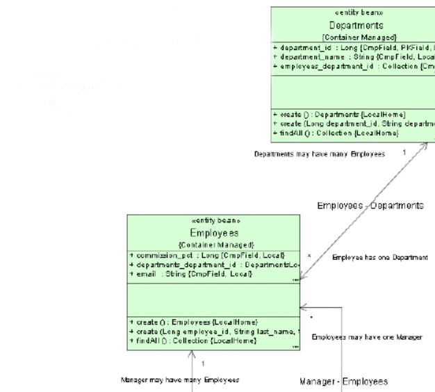
Figure 2-1 JDeveloper-generated UML Diagram with CMR
