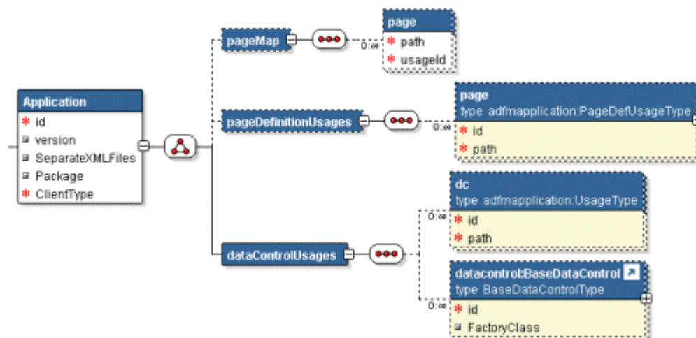
Figure A–9 Schema for the Structure Definition of the DataBindings.cpx File
