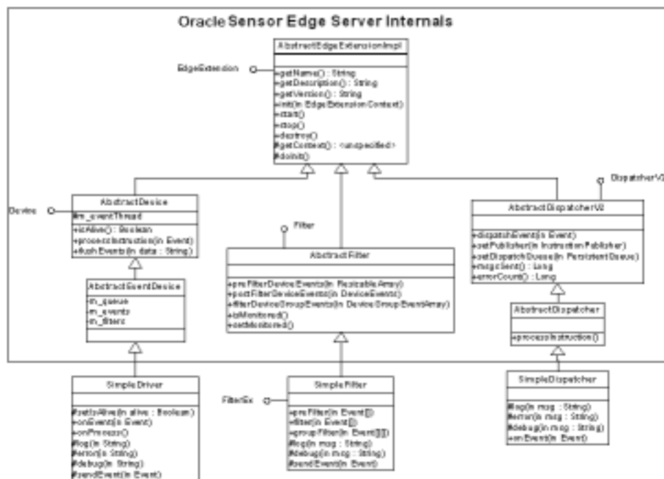
Figure 3–25 The Edge Extension Hierarchy
