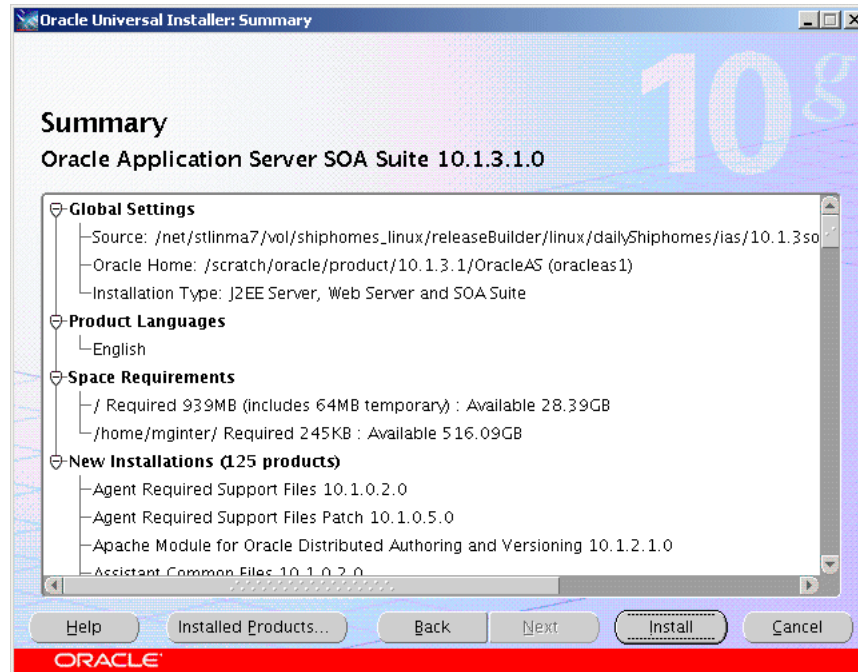
Figure 5–13 Oracle Universal Installer: Summary Screen
