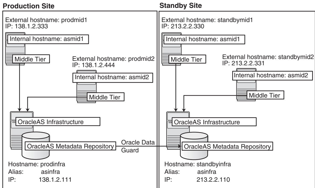
Figure 7-5 OracleAS Disaster Recovery Environment
