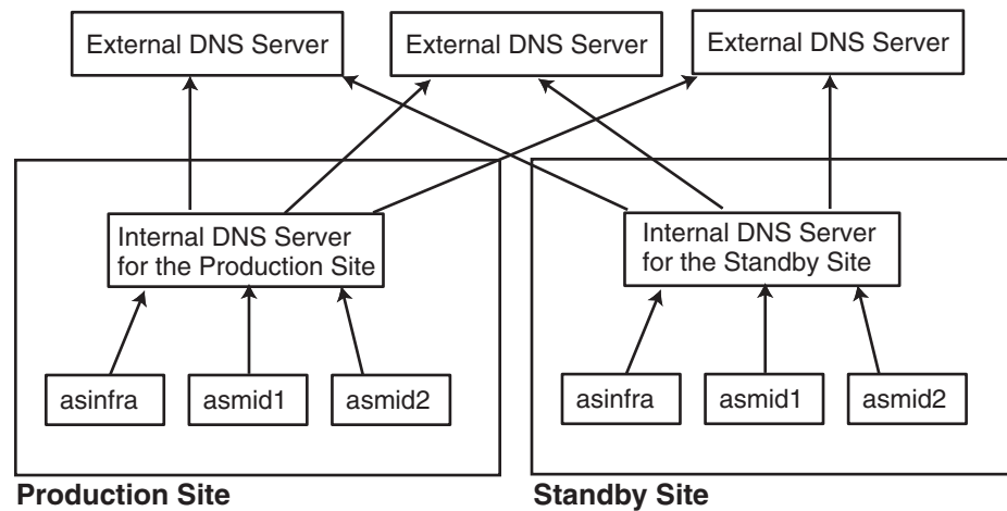
Figure 7-6 Method 1: Using DNS Servers
