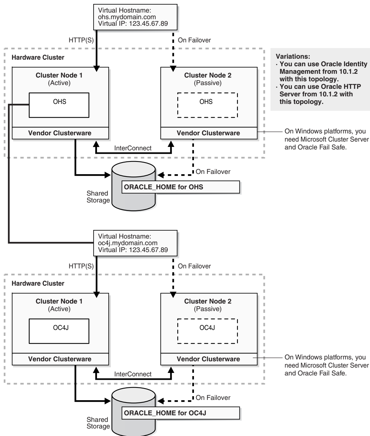
Figure 7–4 Active-Passive Topology with Oracle HTTP Server and OC4J in Separate Oracle Homes
