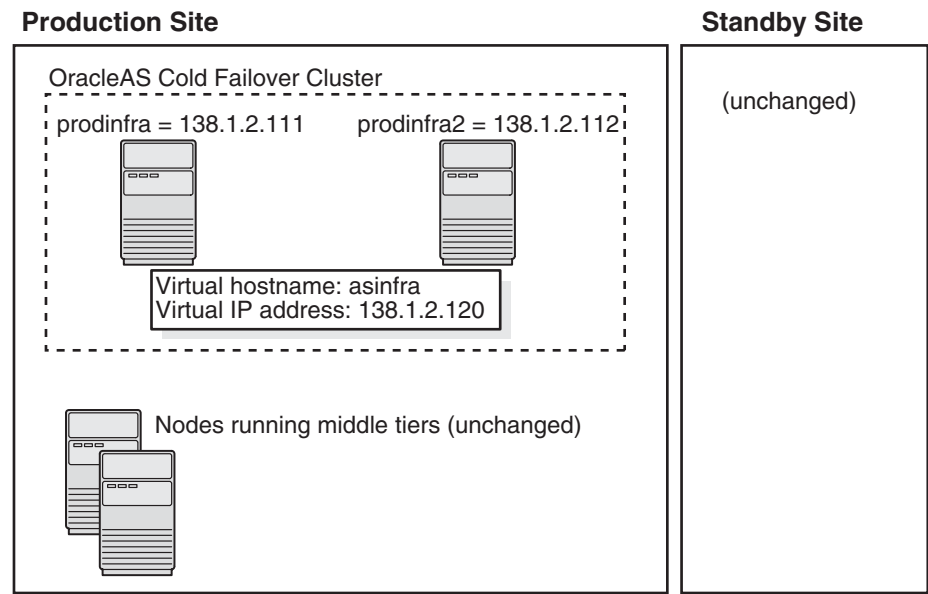
Figure 7-8 Infrastructure in an OracleAS Cold Failover Cluster Configuration
