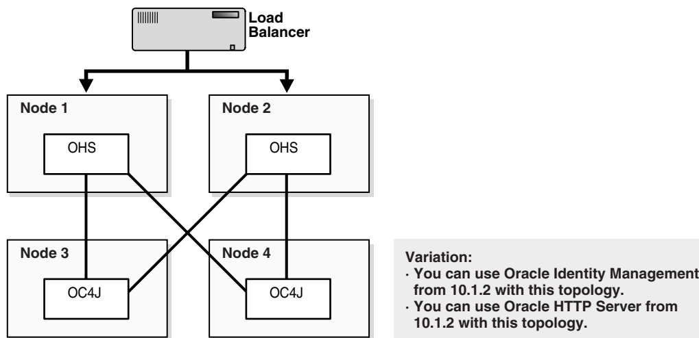
Figure 7–2 Active-Active Topology with Oracle HTTP Server and OC4J in Separate Oracle Homes
