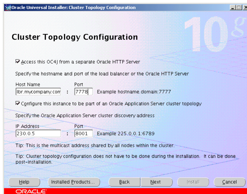
Figure 5–9 Oracle Universal Installer: Cluster Topology Configuration (J2EE Server, Web Server, and SOA Suite Installation)
