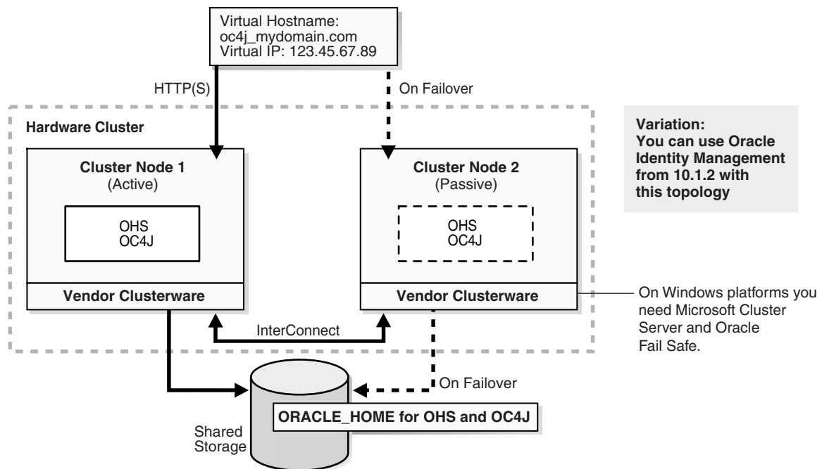
Figure 7-3 Active-Passive Topology with Oracle HTTP Server and OC4J in the Same Oracle Home
