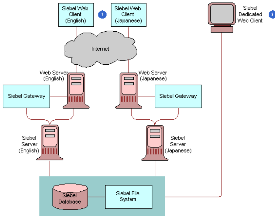
Figure 2. Global Deployment Architecture
