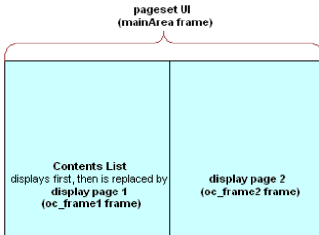
Figure 11. Sample Layout in Which the Contents List is Defined in the Pageset UI Definition File
