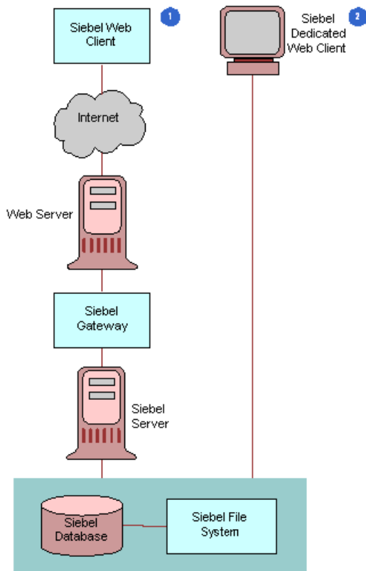
Figure 1. Siebel Advisor Application Architecture
