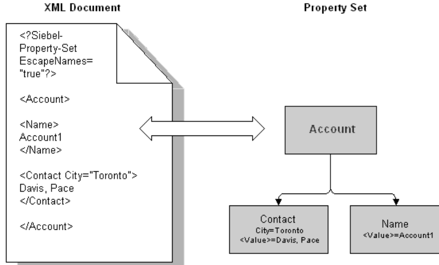
Figure 6. XML Document to Property Set Representation
