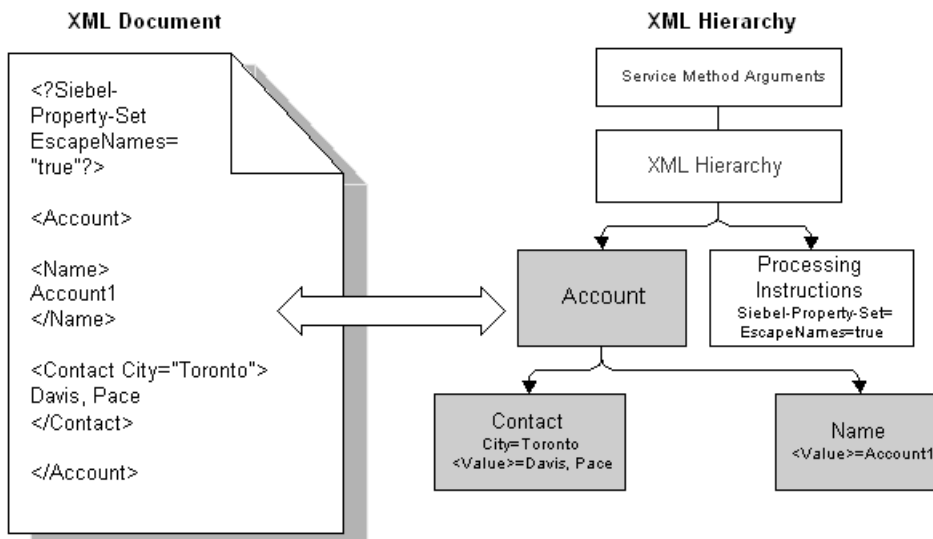
Figure 5. XML Hierarchy Representation of XML Document Structure
